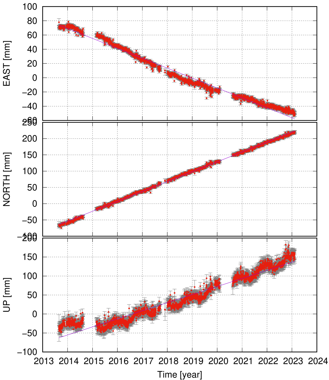
VONC (64.67, -17.75) time series (ITRF 2014) v_e = -13.93 \pm 0.53 ; v_n = 30.39 \pm 0.33 ; v_u = 21.27 \pm 1.54 mm/yr
