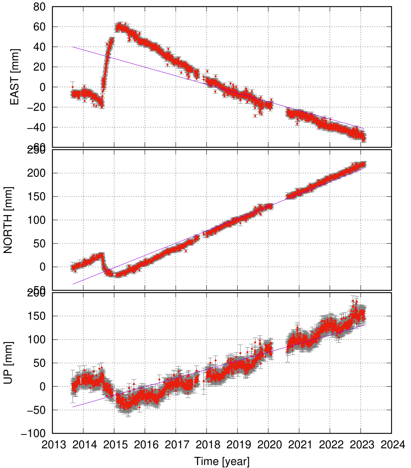
VONC (64.67, -17.75) time series (ITRF 2014) v_e = -8.60 \pm 2.11 ; v_n = 26.14 \pm 1.60 ; v_u = 18.39 \pm 2.42 mm/yr
