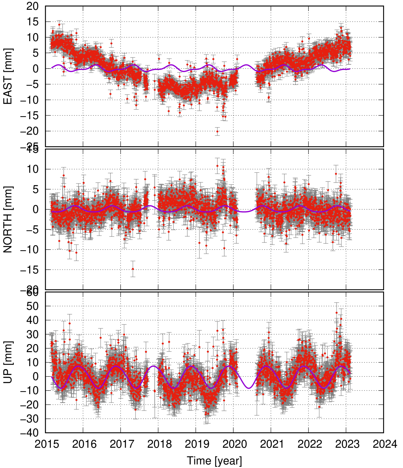
VONC seasonal fit
