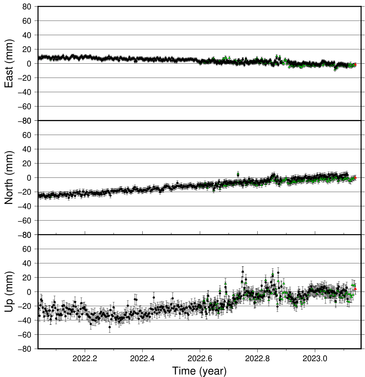
VONC time series (IGS 2014), last 400 days
