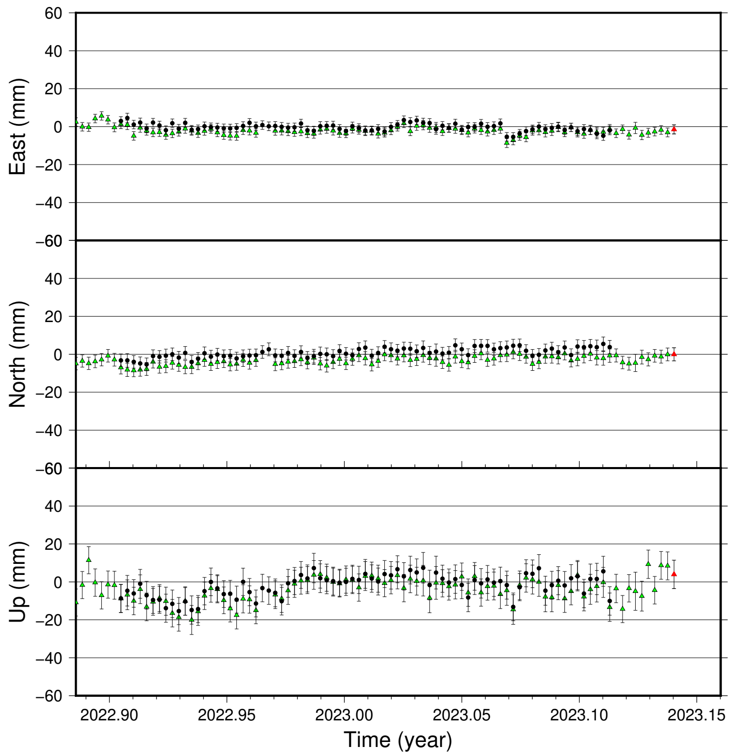
VONC time series (IGS 2014), last 100 days
