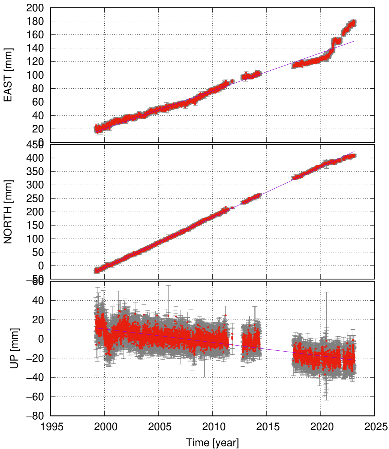
VOGS (63.85, -21.70) time series (ITRF 2014) ve = 5.64 \pm 0.30 ; vn = 18.66 \pm 0.16 ; vu = -1.40 \pm 0.25 mm/yr
