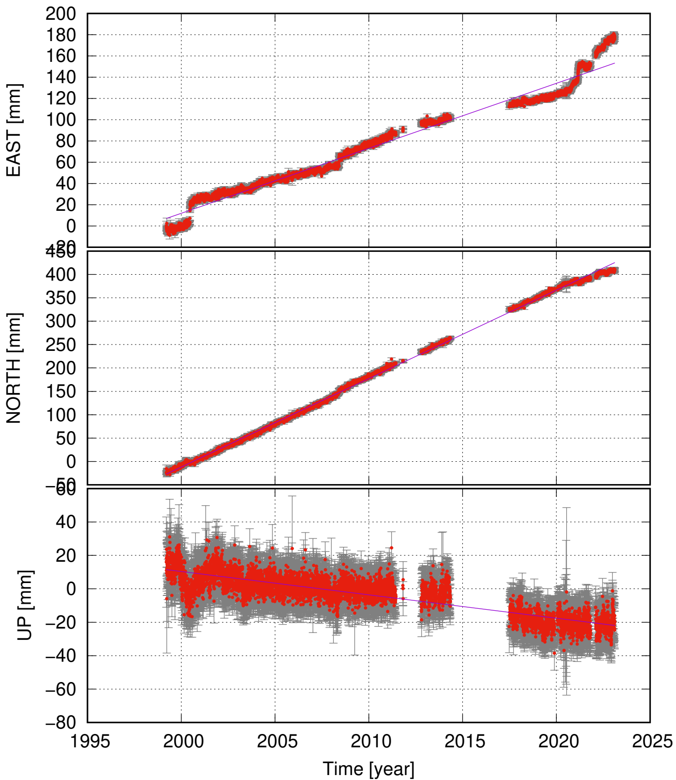
VOGS (63.85, -21.70) time series (ITRF 2014) ve = 6.12 \pm 0.33 ; vn = 18.93 \pm 0.20 ; vu = -1.40 \pm 0.25 mm/yr
