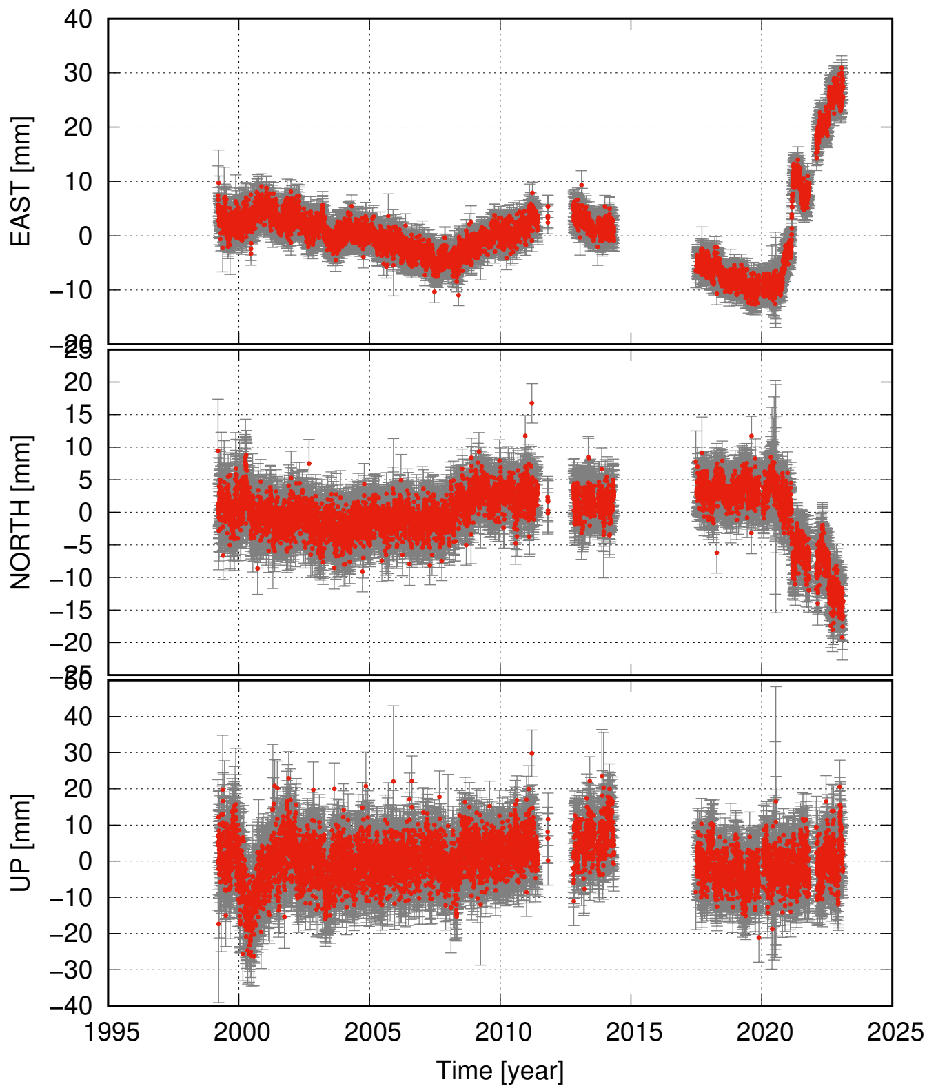
VOGS residual time series (some major events removed as well)
