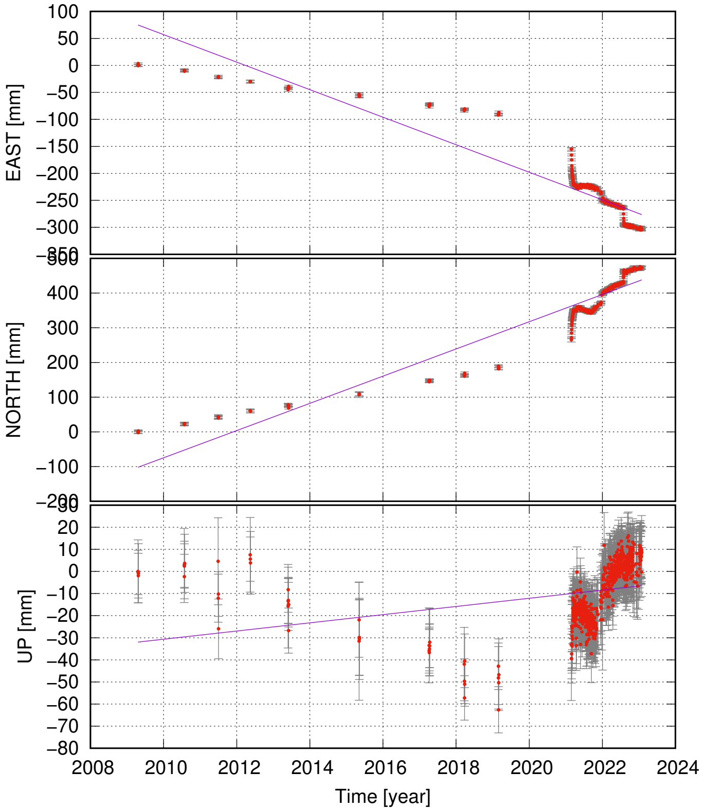
VOGC (63.98, -22.33) time series (ITRF 2014) v_e = -25.49 \pm 1.65 ; v_n = 39.19 \pm 2.37 ; v_u = 1.85 \pm 0.97 mm/yr
