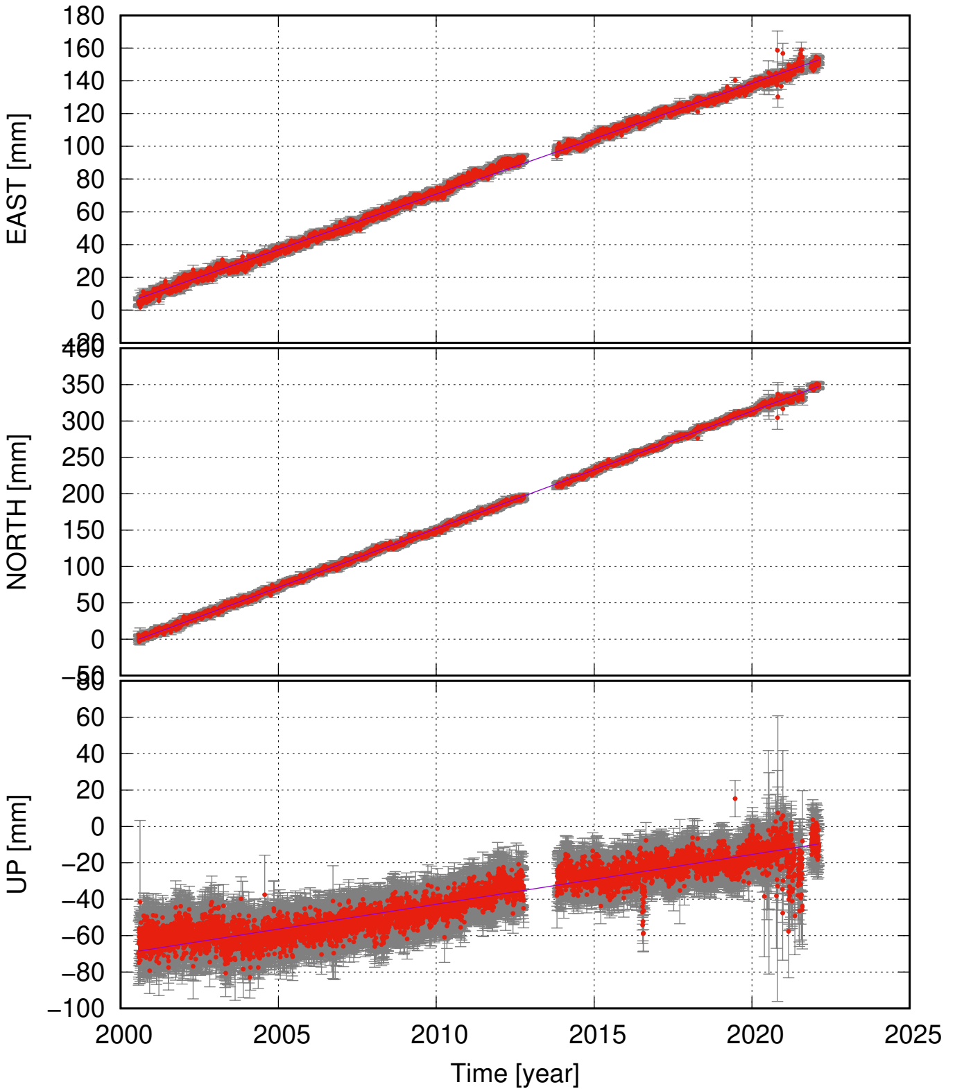
VMEY (63.43, -20.29) time series (ITRF 2014) v_e = 6.76 \pm 0.09 ; v_n = 16.14 \pm 0.10 ; v_u = 2.73 \pm 0.27 mm/yr
