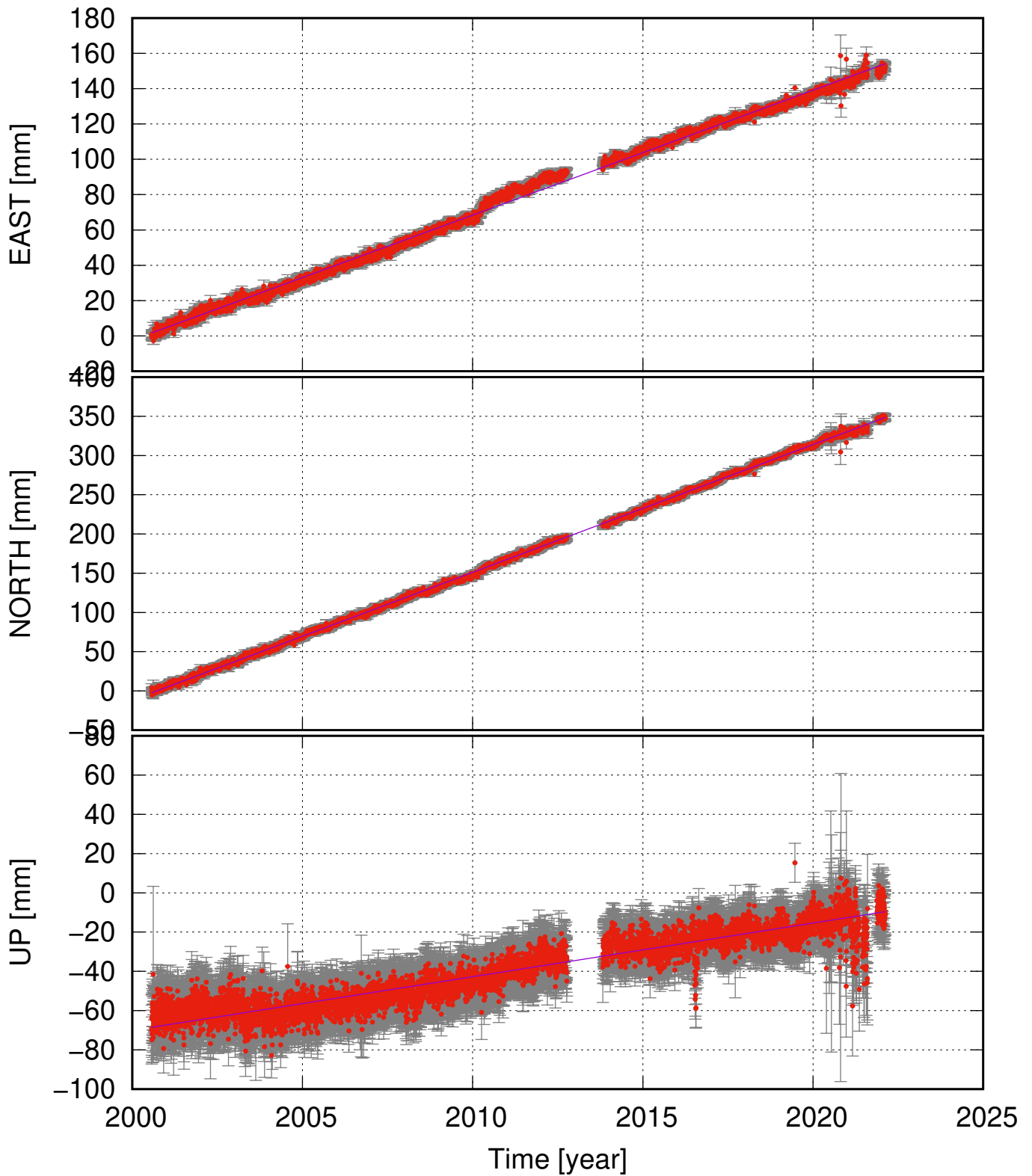
VMEY (63.43, -20.29) time series (ITRF 2014) v_e = 7.07 \pm 0.12 ; v_n = 16.28 \pm 0.10 ; v_u = 2.73 \pm 0.27 mm/yr
