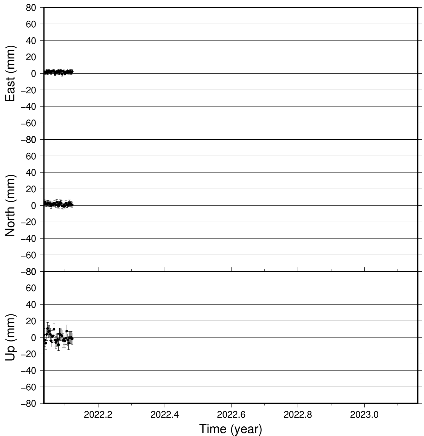
VMEY time series (IGS 2014), last 400 days
