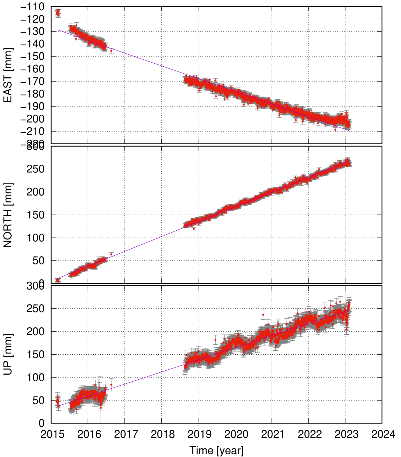
URHC (64.82, -17.15) time series (ITRF 2014) v_e = -10.17 \pm 0.43 ; v_n = 32.33 \pm 0.39 ; v_u = 26.44 \pm 1.12 mm/yr
