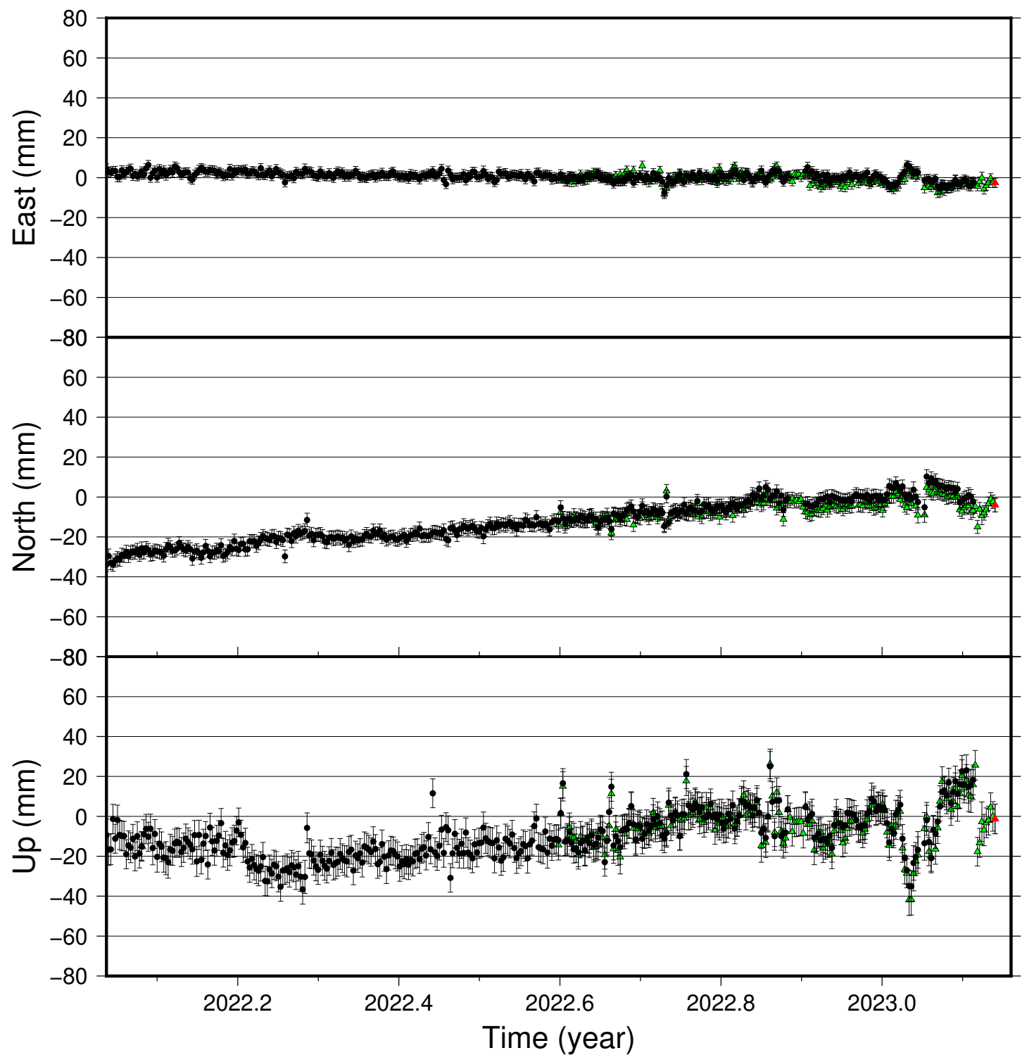
URHC time series (IGS 2014), last 400 days
