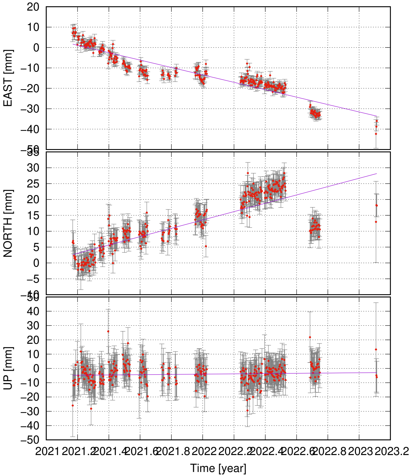
UNDH (63.97, -21.96) time series (ITRF 2014) ve = -18.15 ± 1.98; vn = 13.13 ± 2.52; vu = 0.96 ± 3.41 mm/yr
