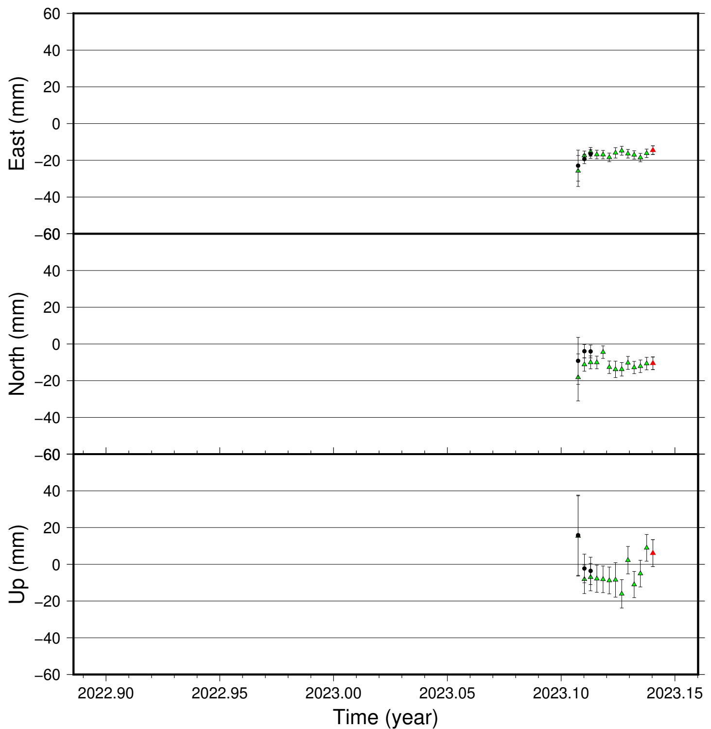
UNDH time series (IGS 2014), last 100 days
