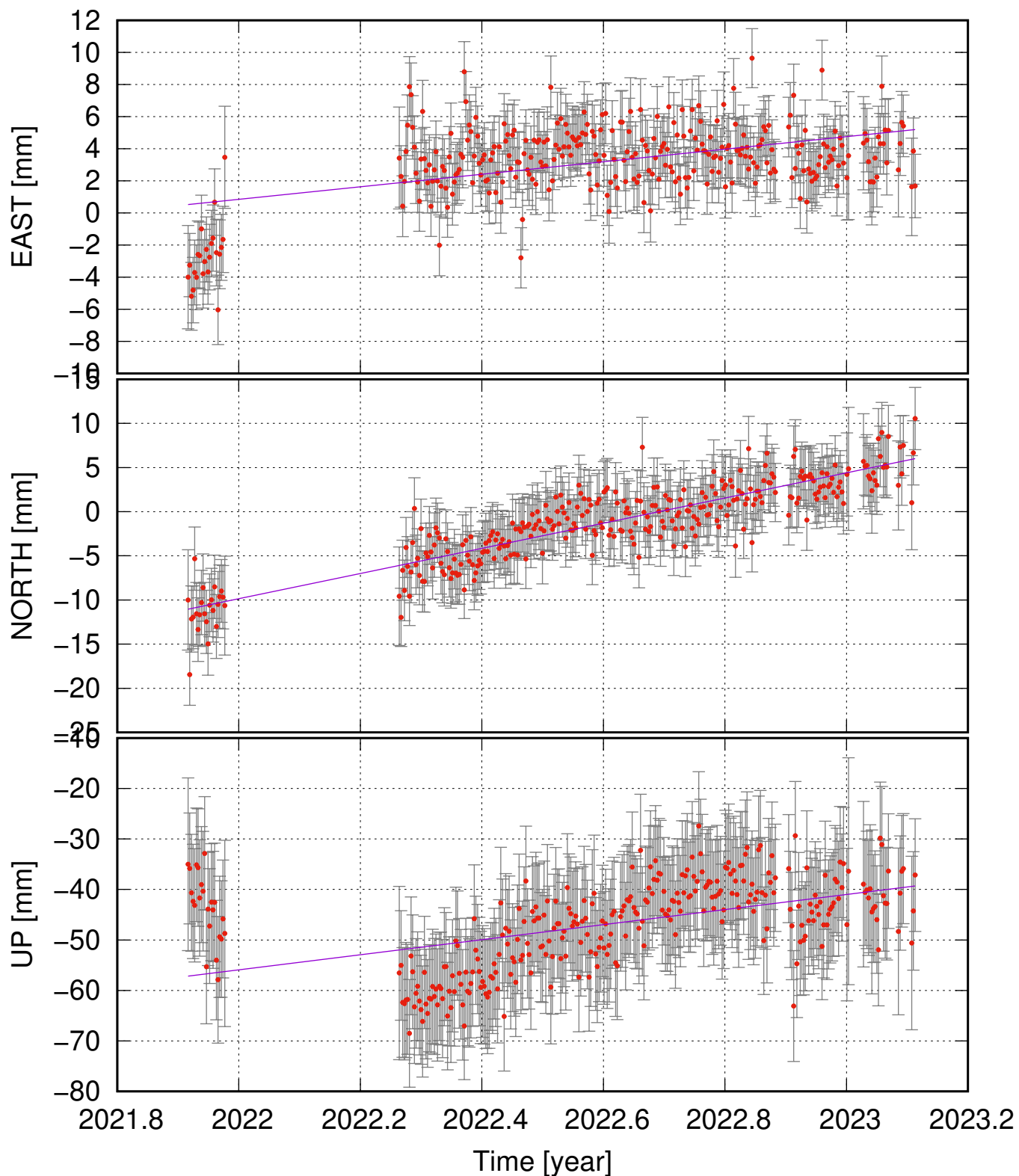
TORK (63.91, -19.07) time series (ITRF 2014) ve = 3.90 \pm 1.75 ; vn = 14.24 \pm 1.81 ; vu = 14.91 \pm 6.40 mm/yr
