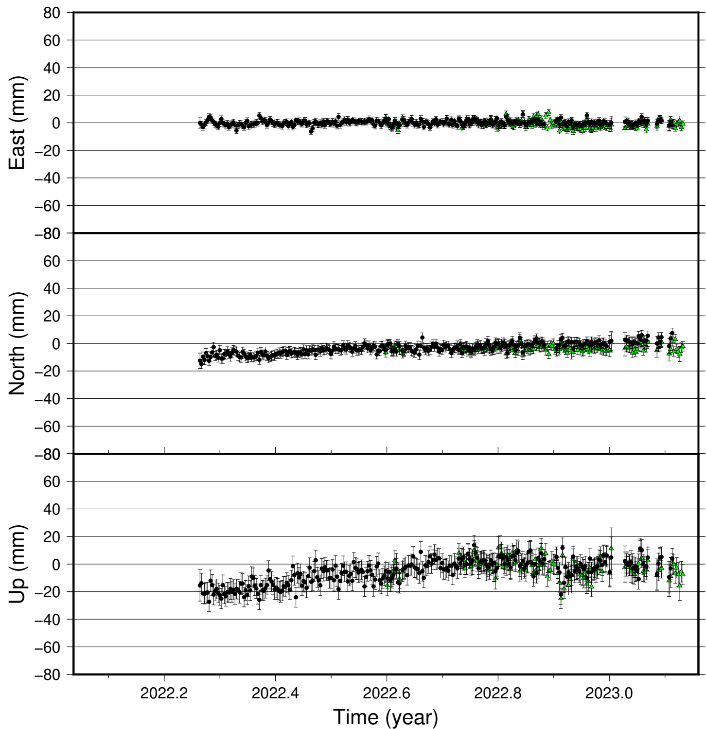
TORK time series (IGS 2014), last 400 days
