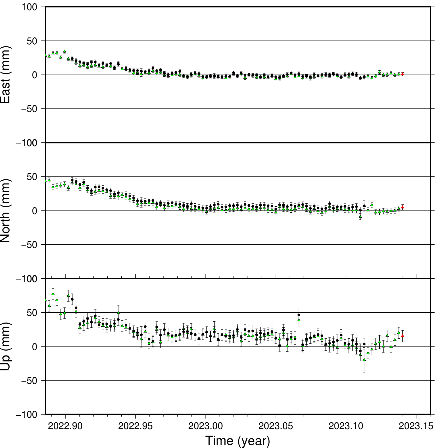
TKJS time series (IGS 2014), last 100 days
