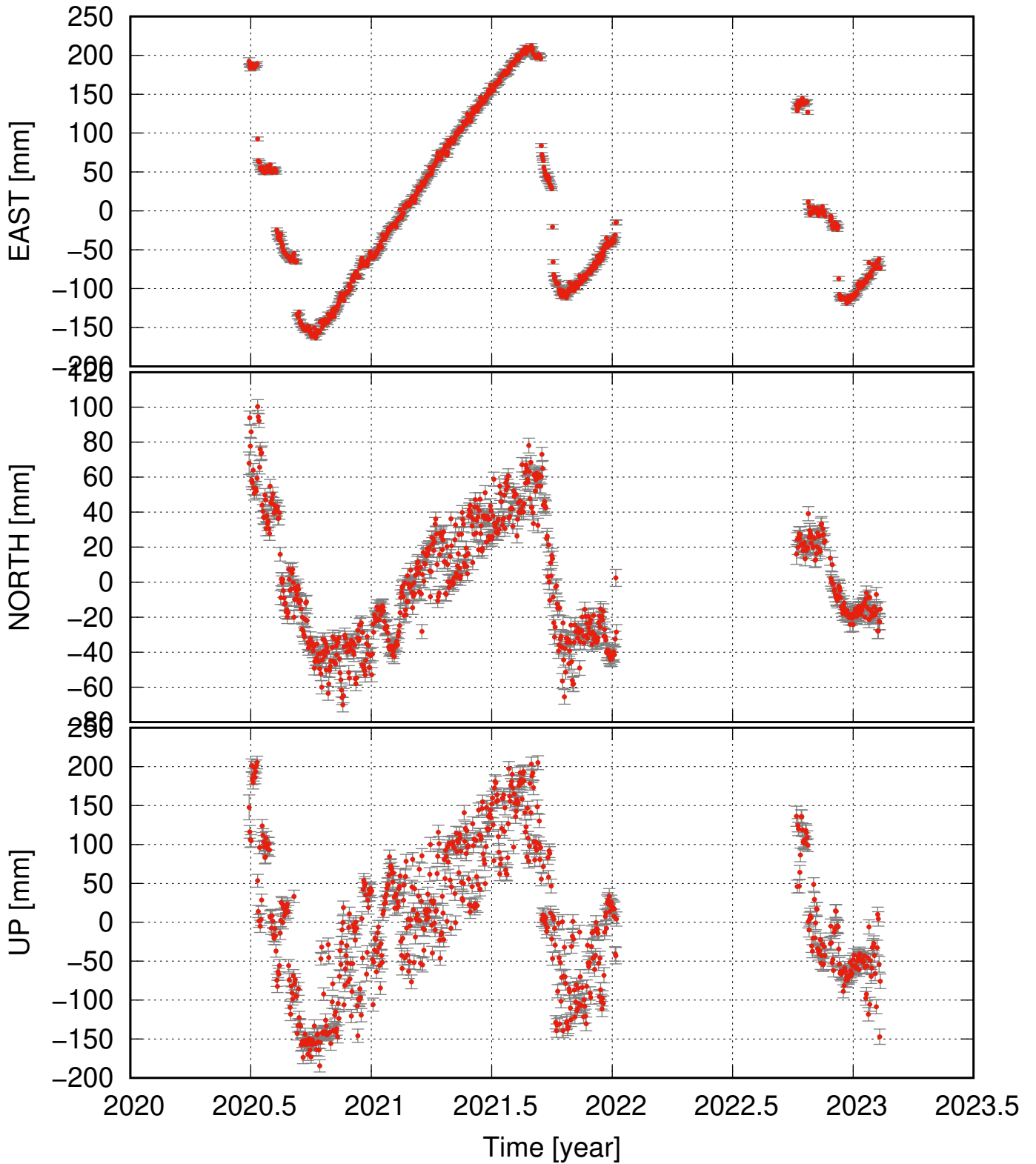
TKJ2 residual time series (some major events removed as well)
