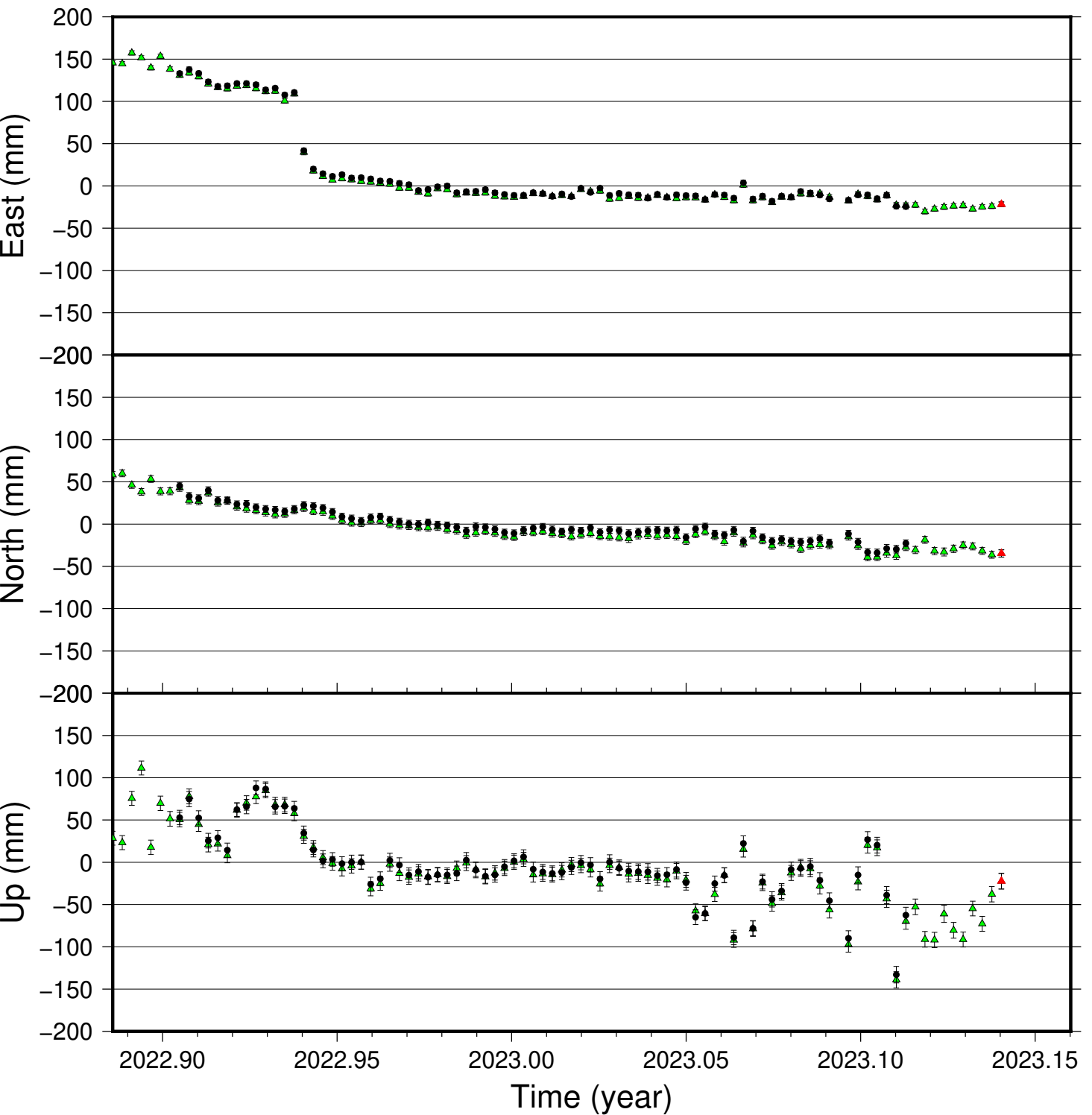
TKJ2 time series (IGS 2014), last 100 days
