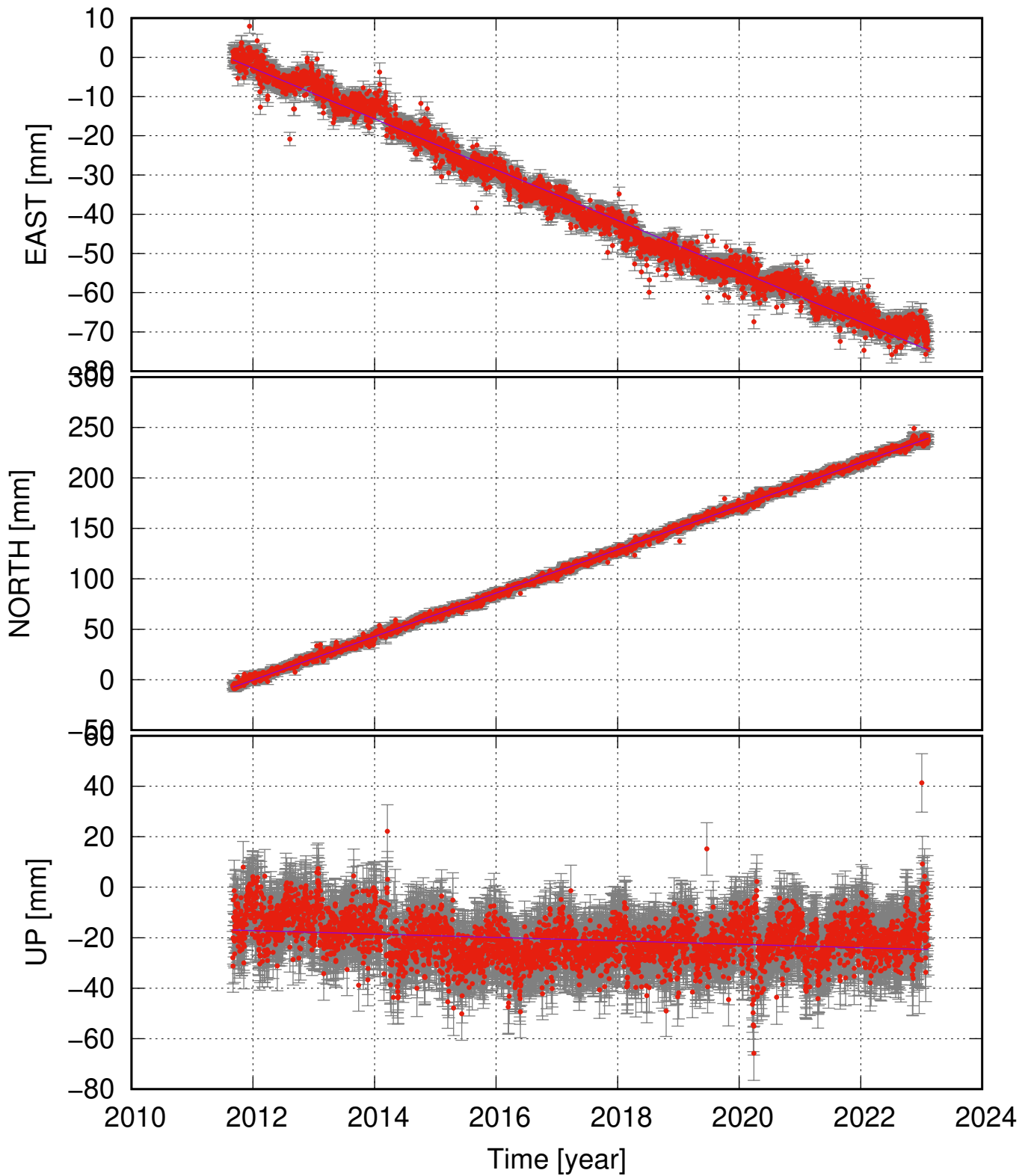
THRC (65.90, -17.01) time series (ITRF 2014) v_e = -6.47 \pm 0.23 ; v_n = 21.57 \pm 0.20 ; v_u = -0.67 \pm 0.70 mm/yr
