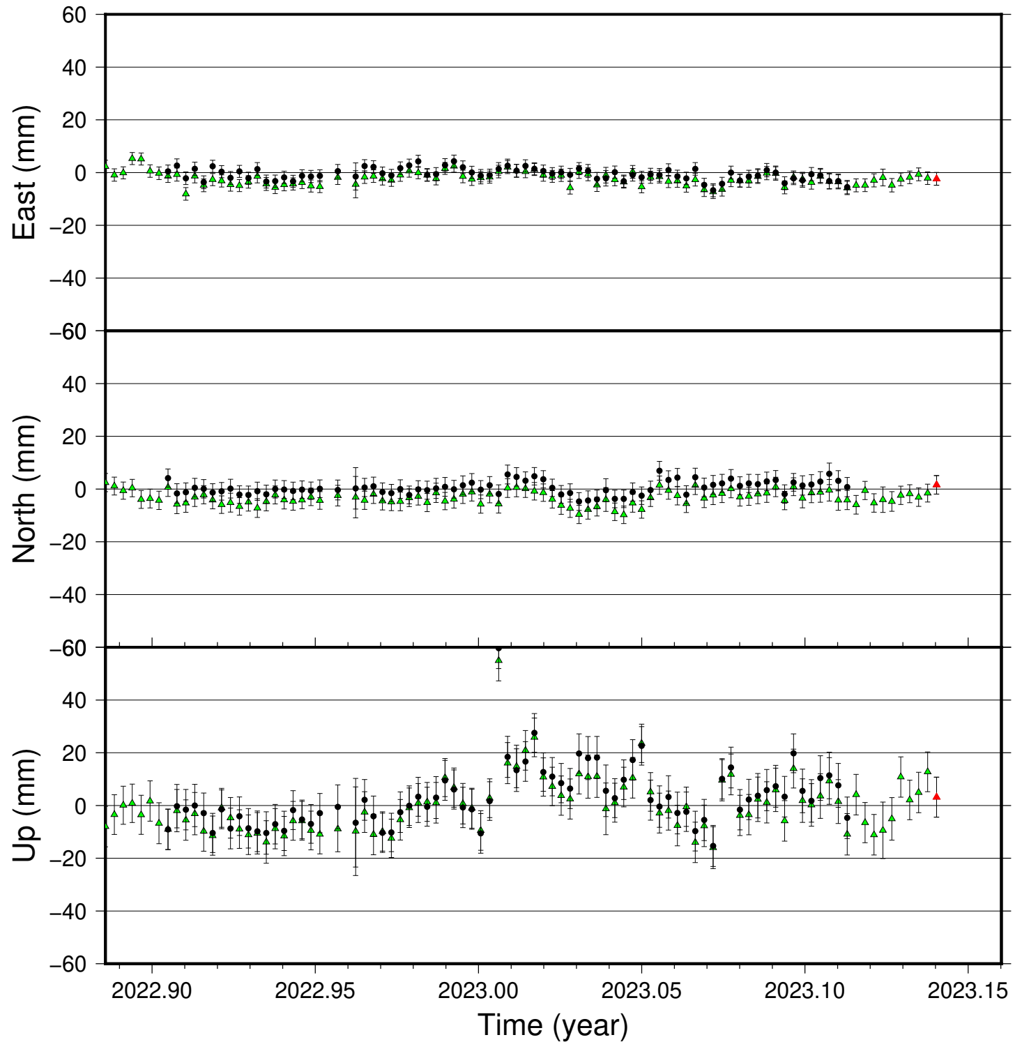
THRC time series (IGS 2014), last 100 days
