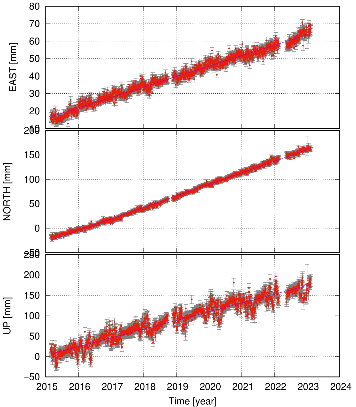
THOC (64.93, -16.68) time series (ITRF 2014) v_e = 5.98 \pm 0.25 ; v_n = 23.62 \pm 0.38 ; v_u = 21.41 \pm 1.69 mm/yr
