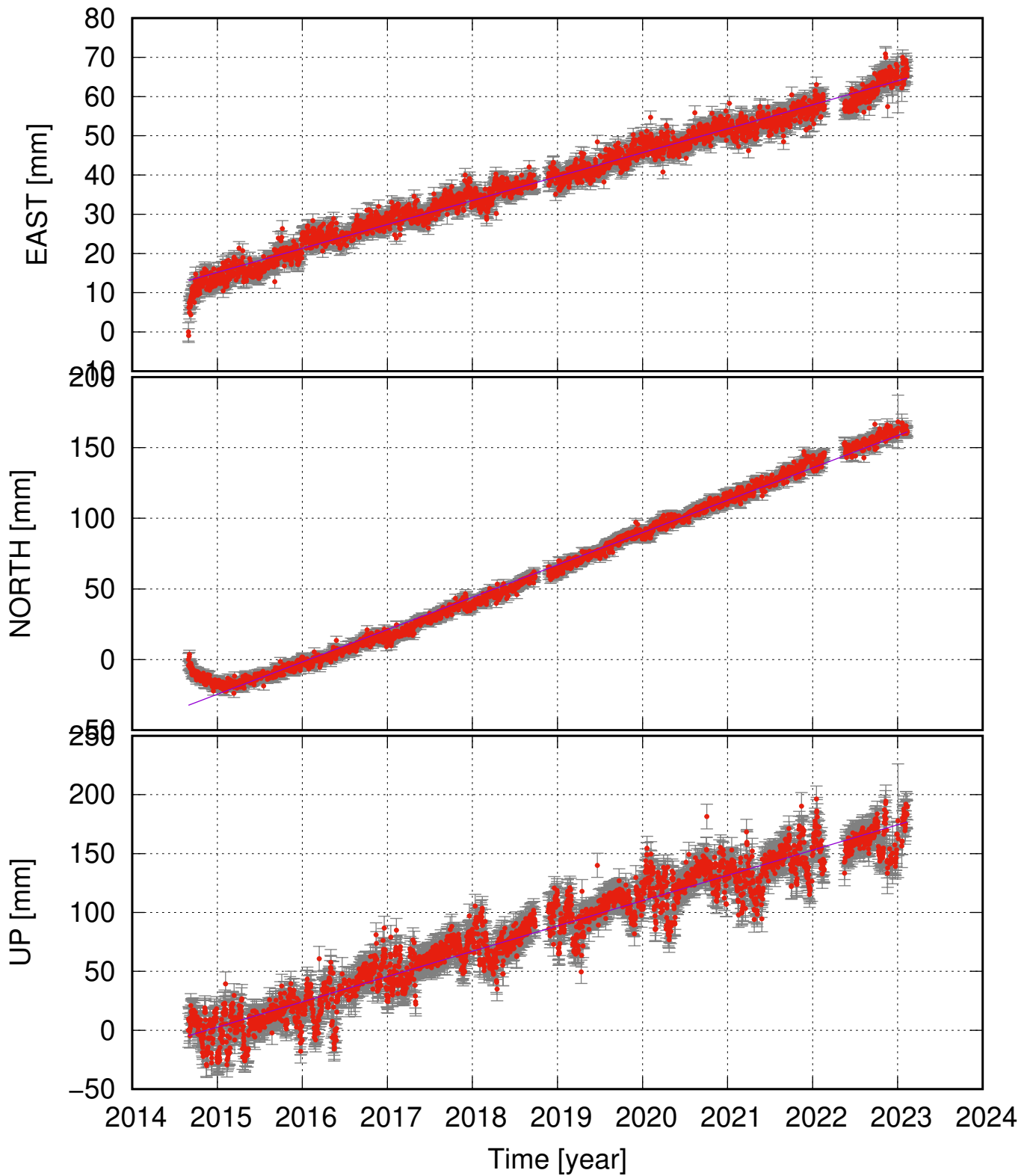
THOC (64.93, -16.68) time series (ITRF 2014) v_e = 6.10 \pm 0.24 ; v_n = 22.90 \pm 0.60 ; v_u = 21.47 \pm 1.60 mm/yr
