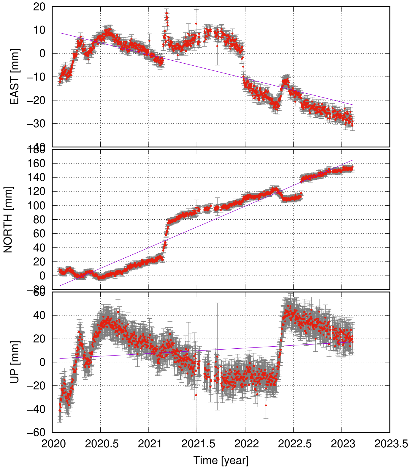
THOB (63.86, -22.44) time series (ITRF 2014) v_e = -10.14 \pm 2.63 ; v_n = 59.02 \pm 4.72 ; v_u = 4.65 \pm 6.51 mm/yr
