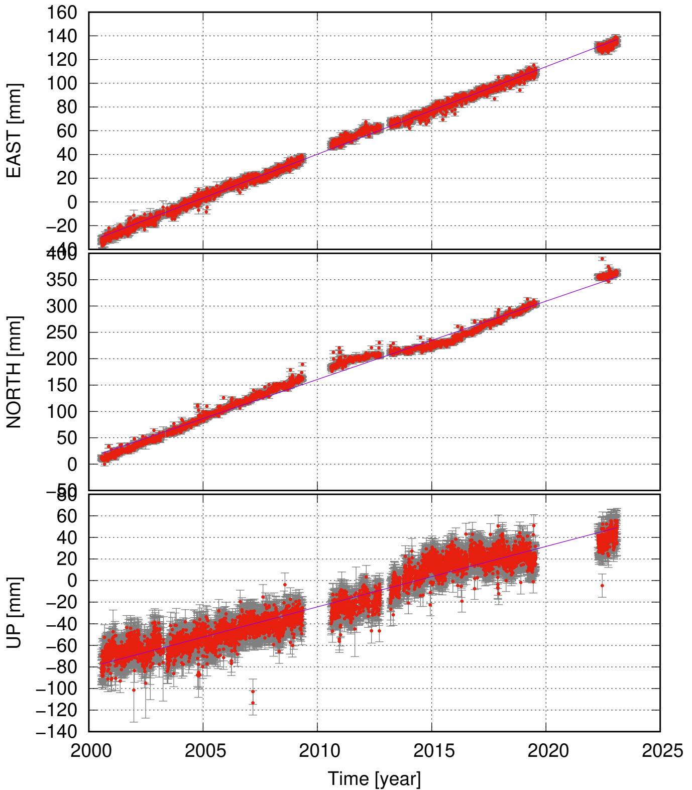
THEY (63.56, -19.64) time series (ITRF 2014) v_e = 7.38 \pm 0.11 ; v_n = 14.85 \pm 0.40 ; v_u = 5.60 \pm 0.39 mm/yr
