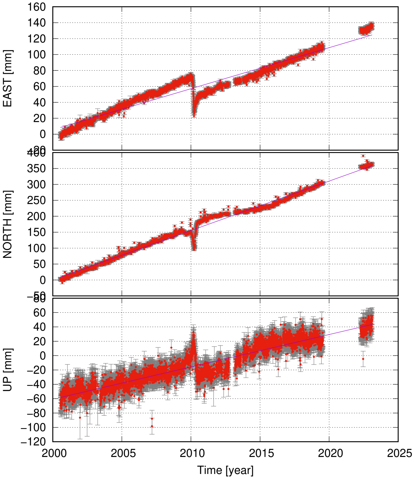
THEY (63.56, -19.64) time series (ITRF 2014) v_e = 5.15 \pm 0.35 ; v_n = 15.50 \pm 0.44 ; v_u = 4.52 \pm 0.43 mm/yr
