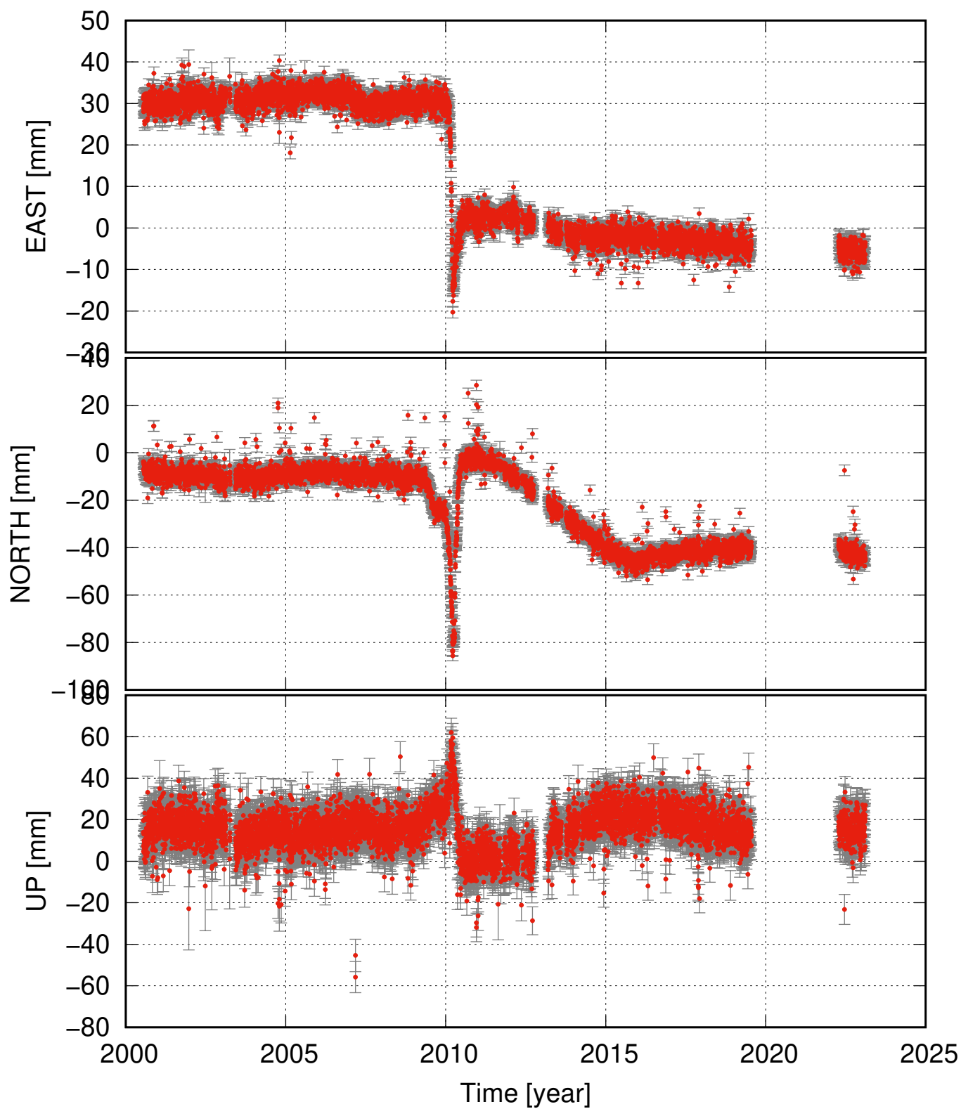
THEY detrended and seasonal signal removed
