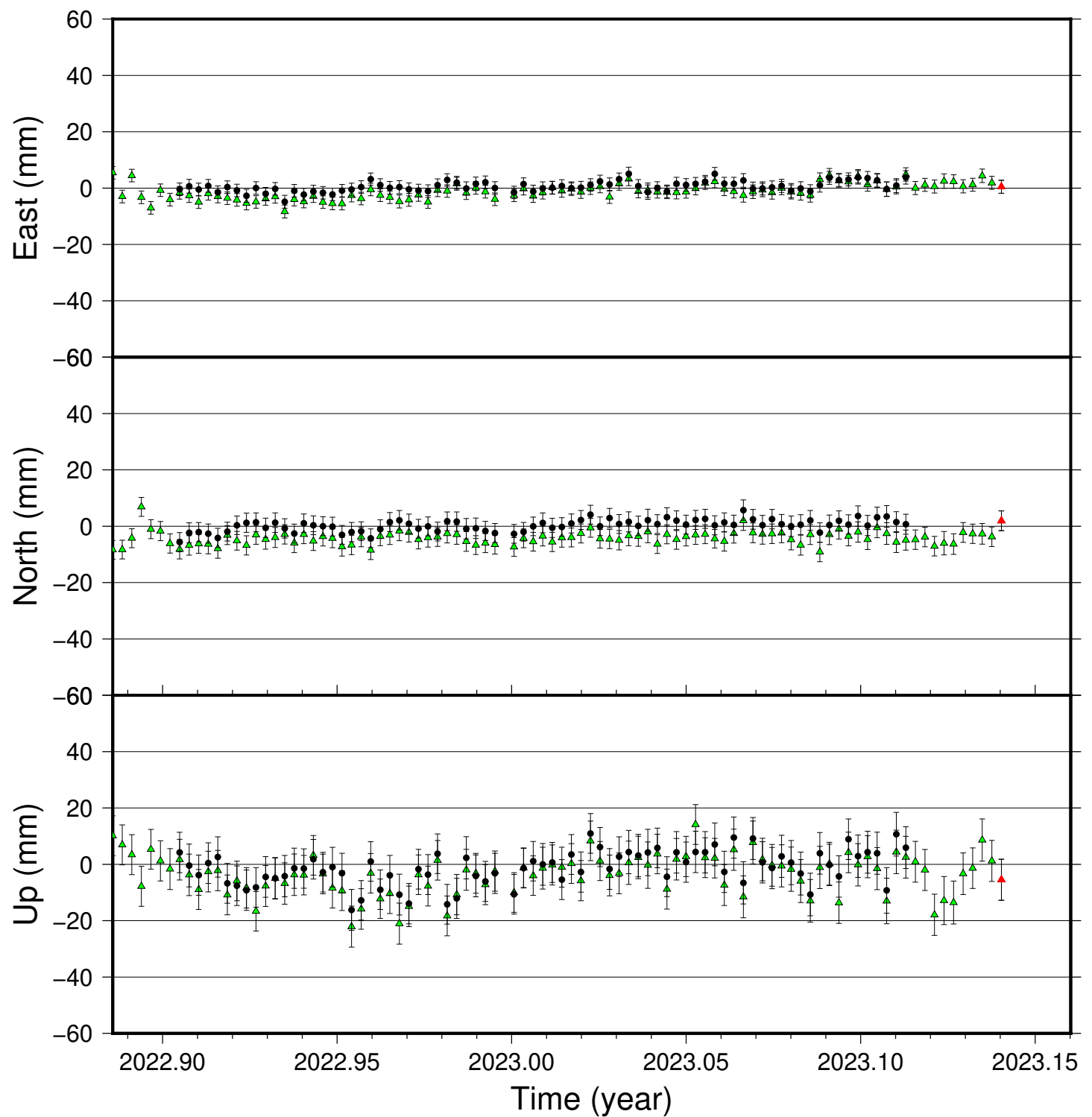
THEY time series (IGS 2014), last 100 days
