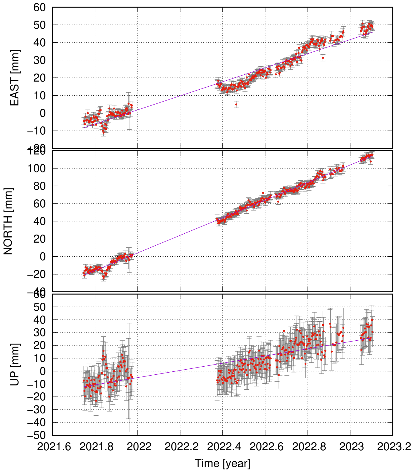
TANC (65.08, -16.74) time series (ITRF 2014) v_e = 39.86 \pm 2.81 ; v_n = 99.62 \pm 2.26 ; v_u = 28.06 \pm 6.12 mm/yr
