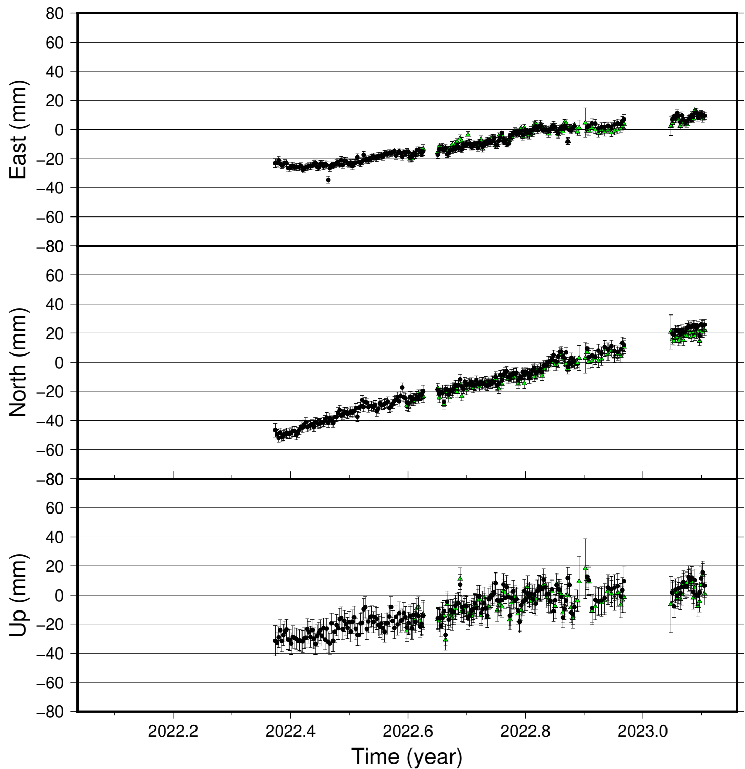
TANC time series (IGS 2014), last 400 days
