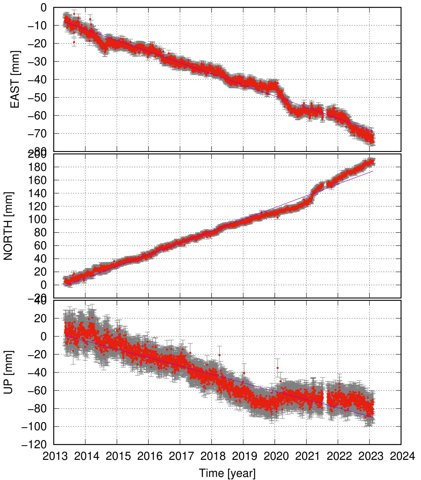
SYRF (63.84, -22.65) time series (ITRF 2014) v_e = -6.18 \pm 0.26 ; v_n = 17.97 \pm 0.67 ; v_u = -9.31 \pm 0.95 mm/yr
