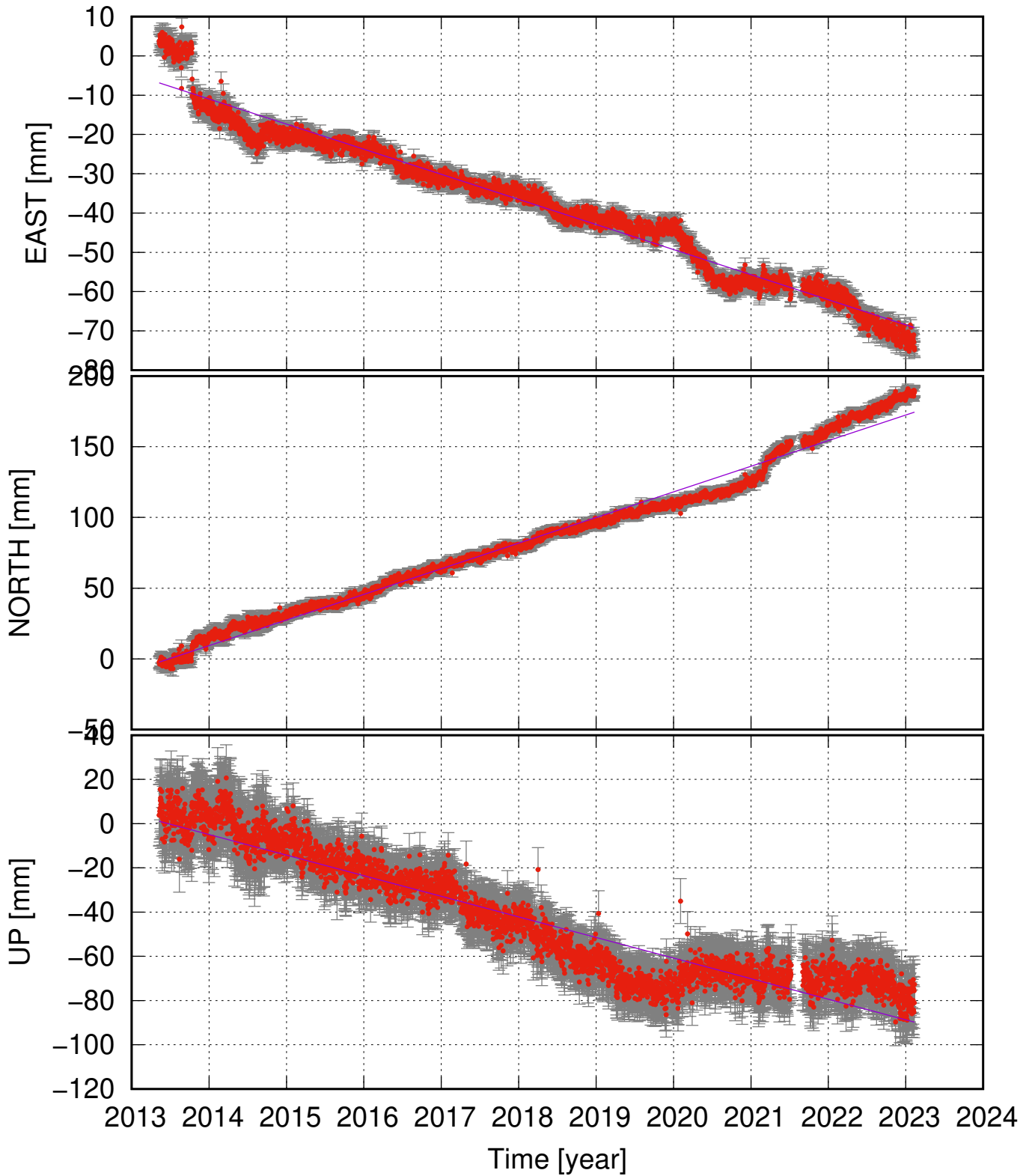
SYRF (63.84, -22.65) time series (ITRF 2014) v_e = -6.39 \pm 0.35 ; v_n = 18.11 \pm 0.66 ; v_u = -9.31 \pm 0.95 mm/yr
