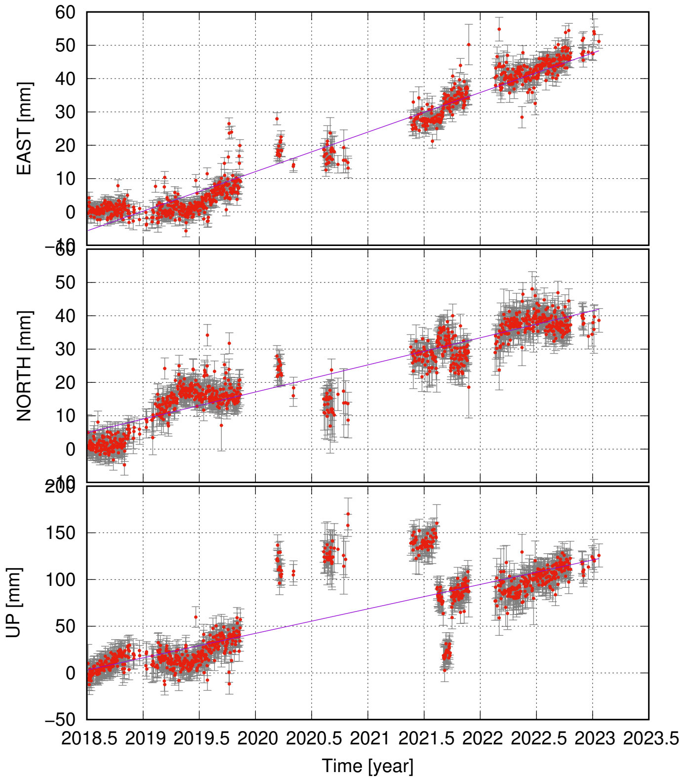
SVIN (64.01, -16.82) time series (ITRF 2014) ve = 11.87 \pm 0.84 ; vn = 8.14 \pm 1.02 ; vu = 26.20 \pm 5.89 mm/yr
