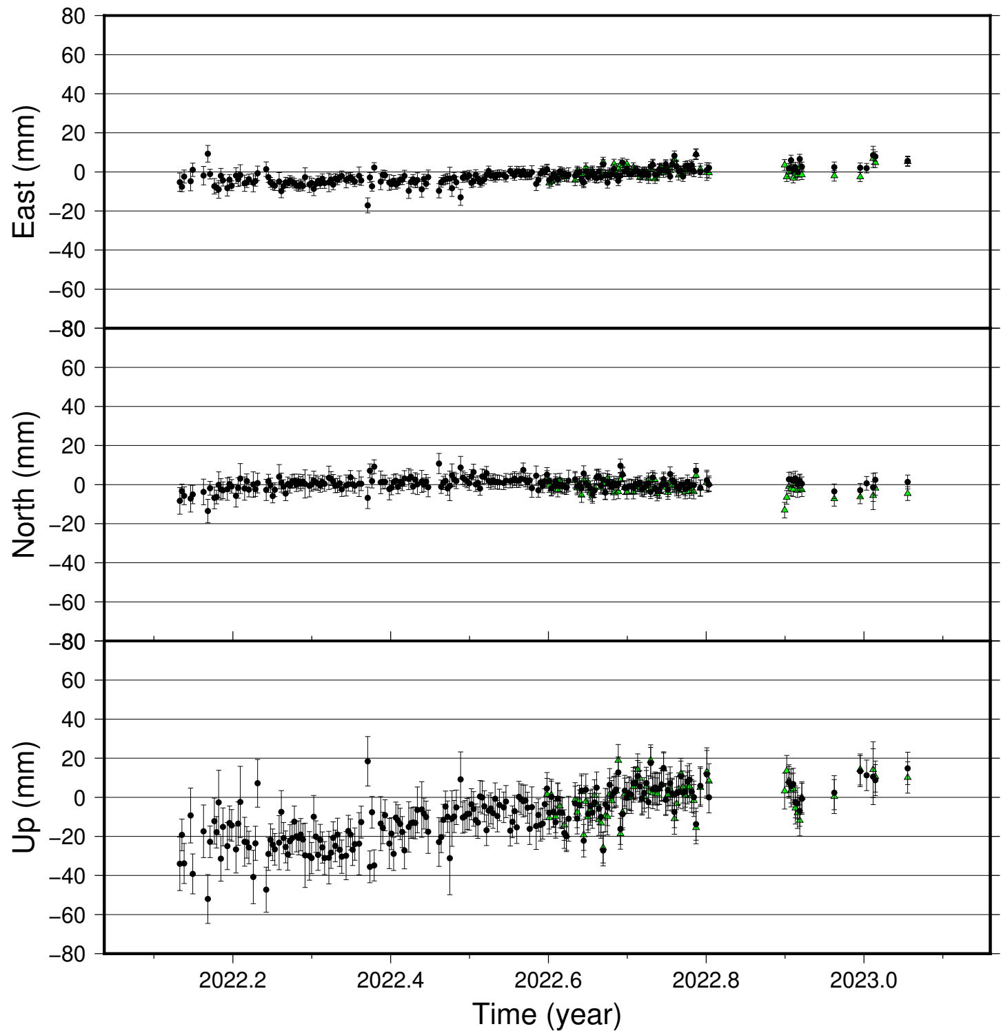
SVIN time series (IGS 2014), last 400 days
