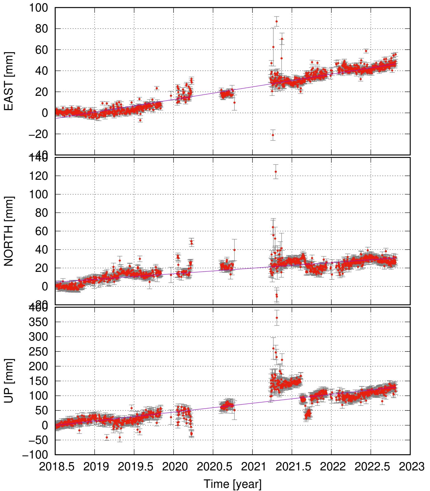
SVIE (64.01, -16.80) time series (ITRF 2014) v_e = 12.01 \pm 1.13 ; v_n = 6.09 \pm 1.53 ; v_u = 30.10 \pm 6.74 mm/yr
