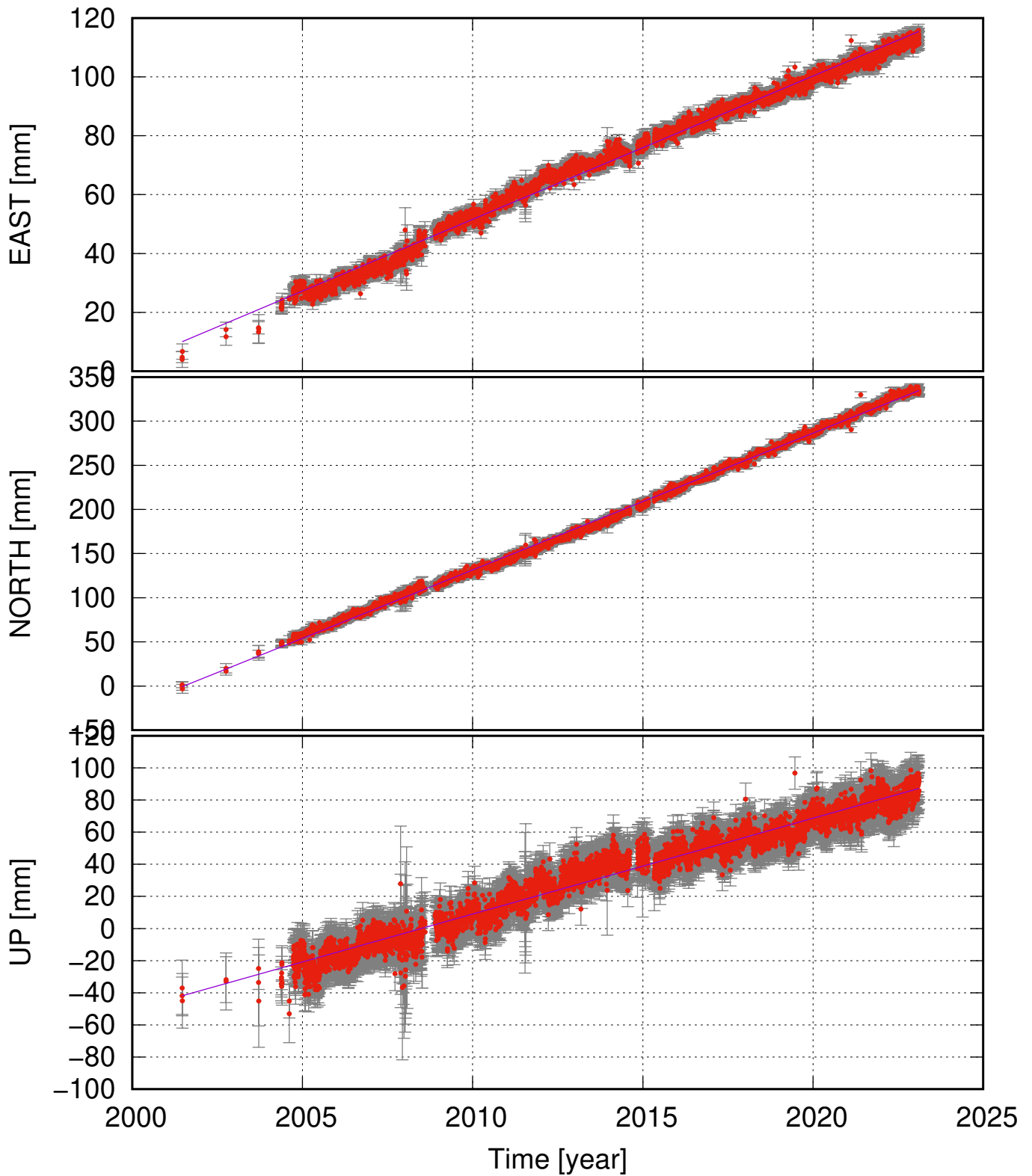
STOR (63.75, -20.21) time series (ITRF 2014) v_e = 4.87 \pm 0.11 ; v_n = 15.50 \pm 0.16 ; v_u = 5.97 \pm 0.29 mm/yr
