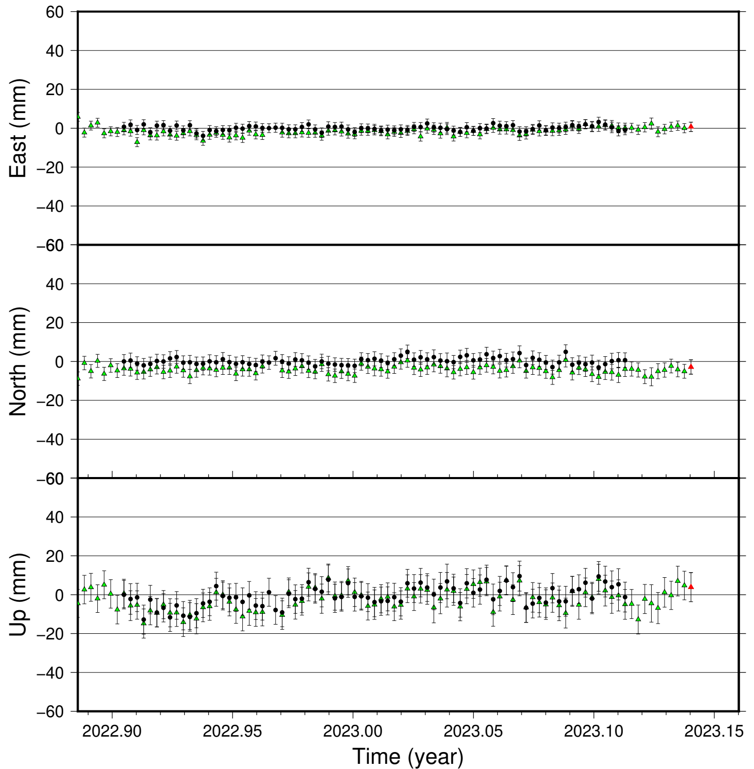
STOR time series (IGS 2014), last 100 days
