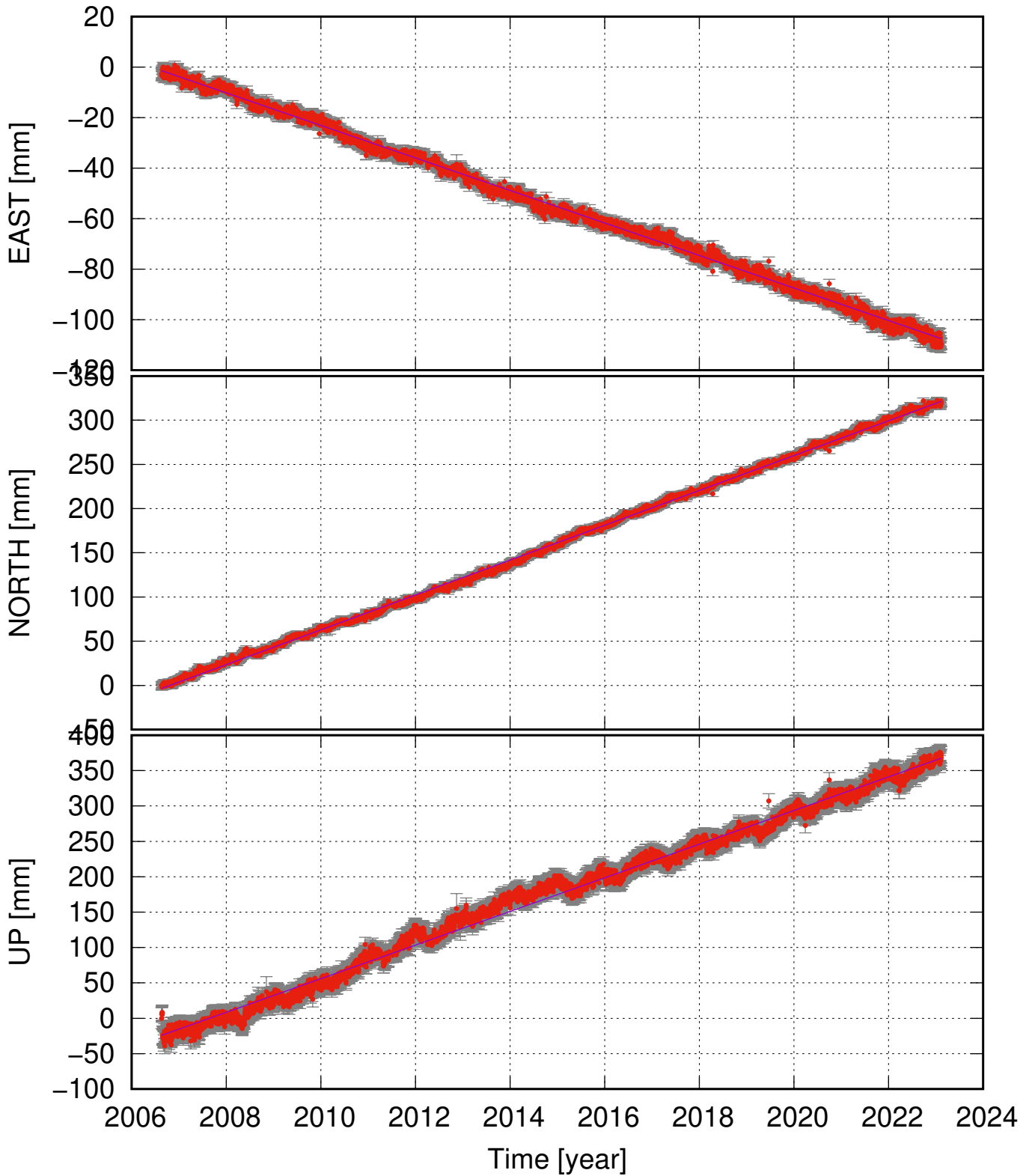
STKA (64.44, -18.82) time series (ITRF 2014) v_e = -6.44 \pm 0.10 ; v_n = 19.72 \pm 0.18 ; v_u = 23.77 \pm 0.59 mm/yr
