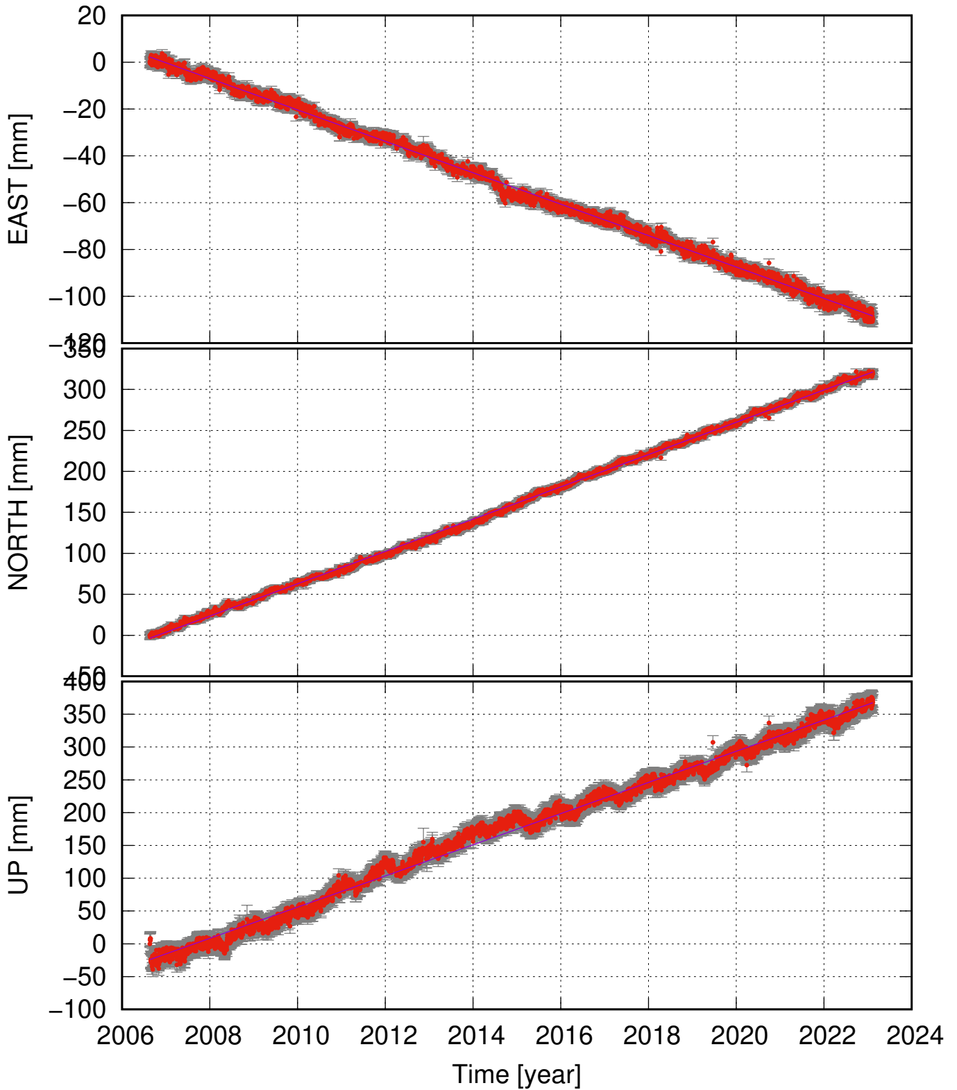
STKA (64.44, -18.82) time series (ITRF 2014) v_e = -6.71 \pm 0.10 ; v_n = 19.72 \pm 0.18 ; v_u = 23.77 \pm 0.59 mm/yr
