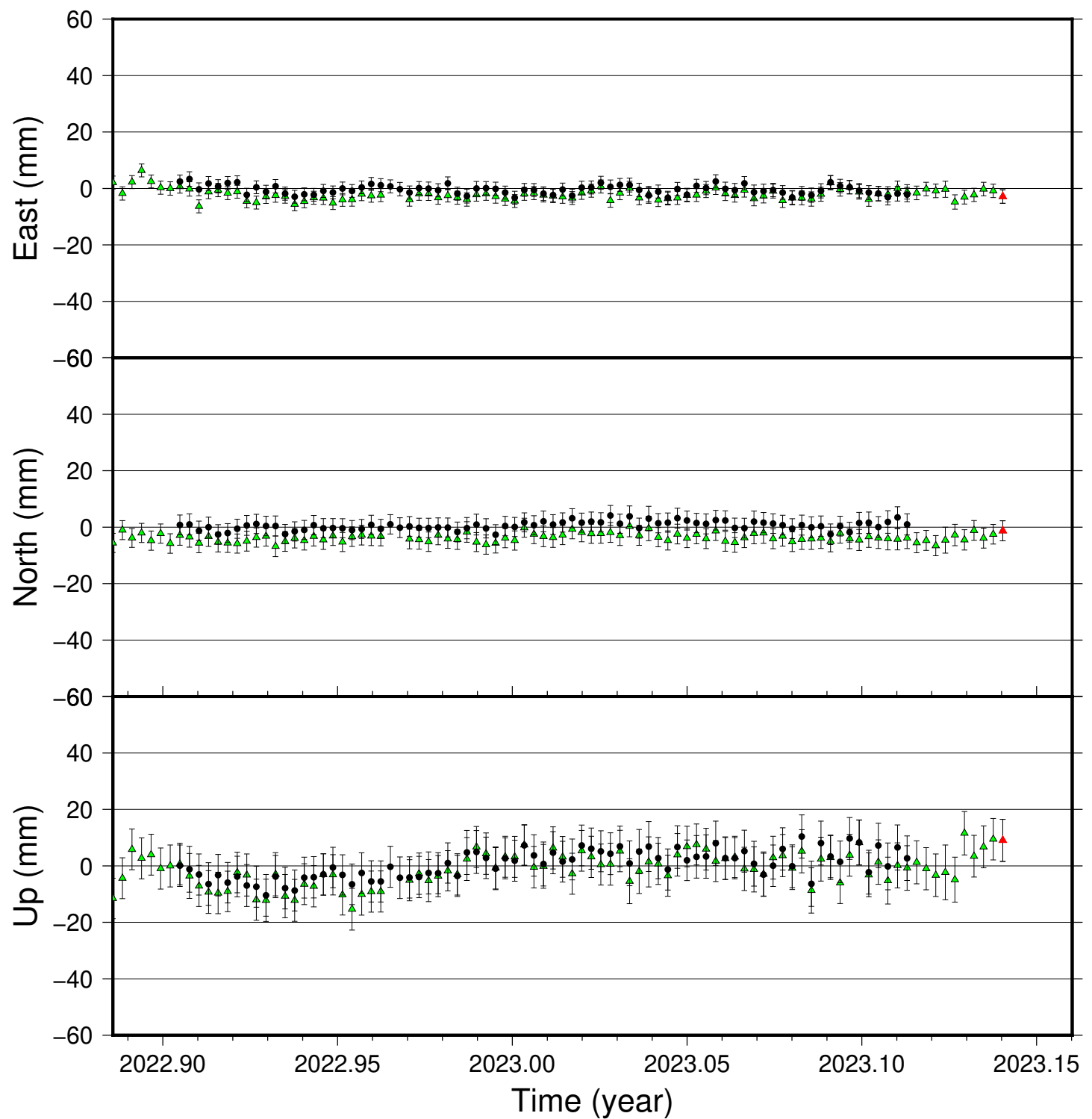
STKA time series (IGS 2014), last 100 days
