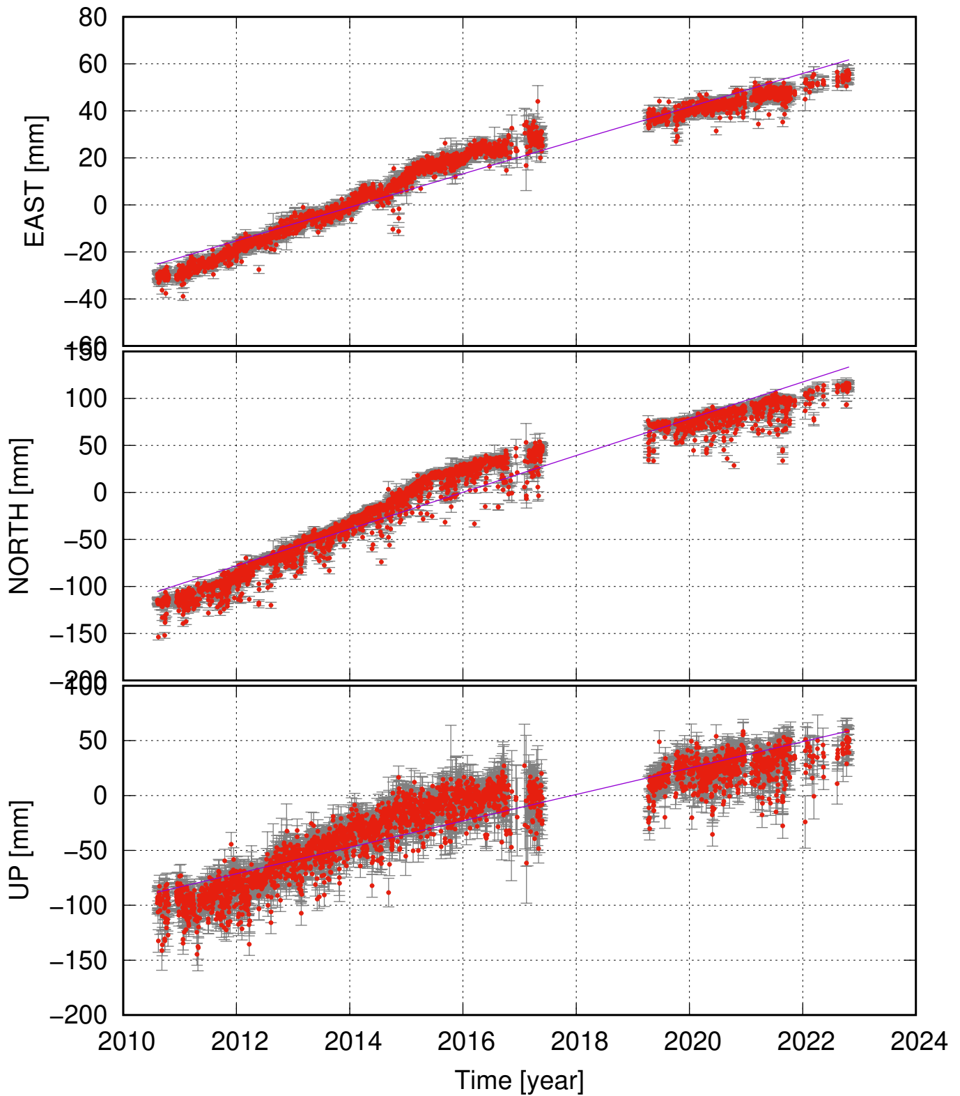
STE2 (63.68, -19.61) time series (ITRF 2014) v_e = 7.12 \pm 0.42 ; v_n = 19.54 \pm 1.32 ; v_u = 12.03 \pm 1.43 mm/yr
