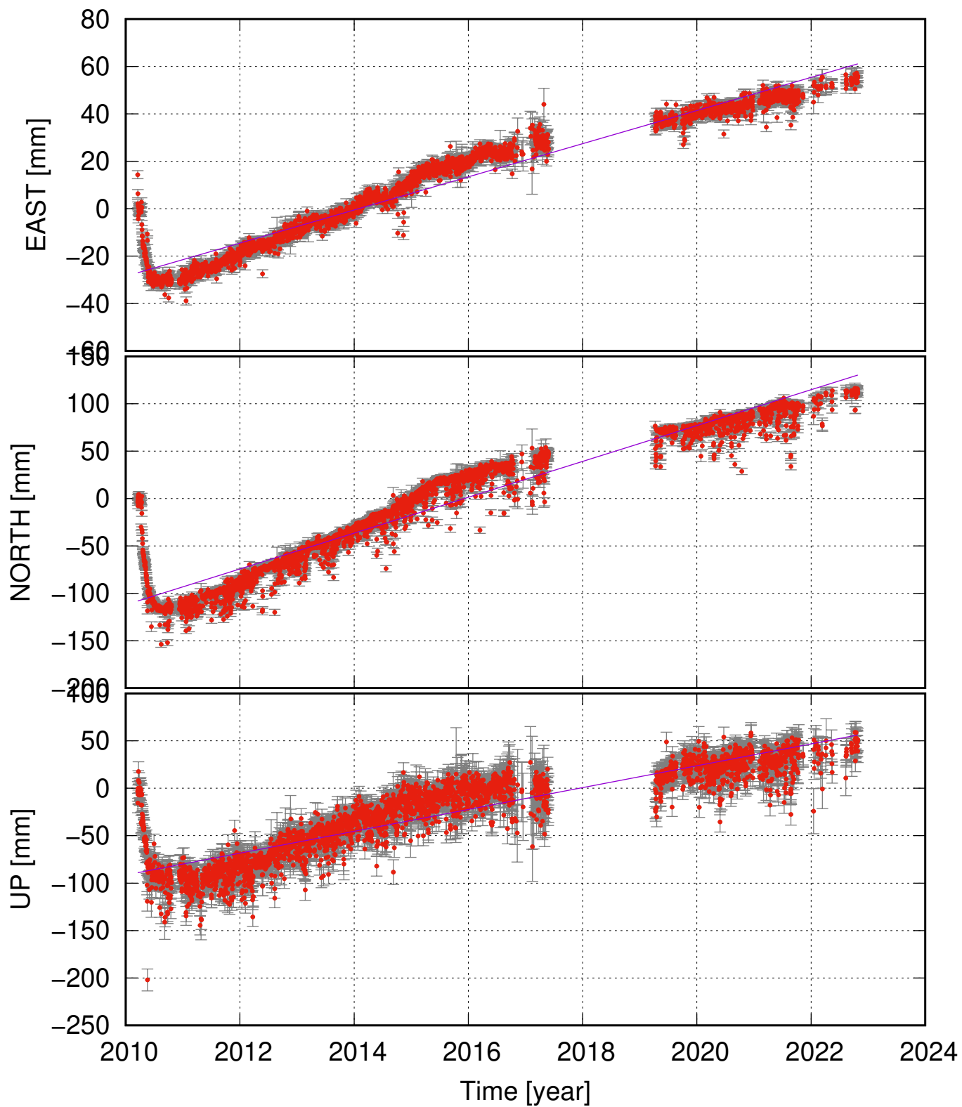
STE2 (63.68, -19.61) time series (ITRF 2014) v_e = 6.99 \pm 0.46 ; v_n = 18.89 \pm 1.53 ; v_u = 11.52 \pm 1.55 mm/yr
