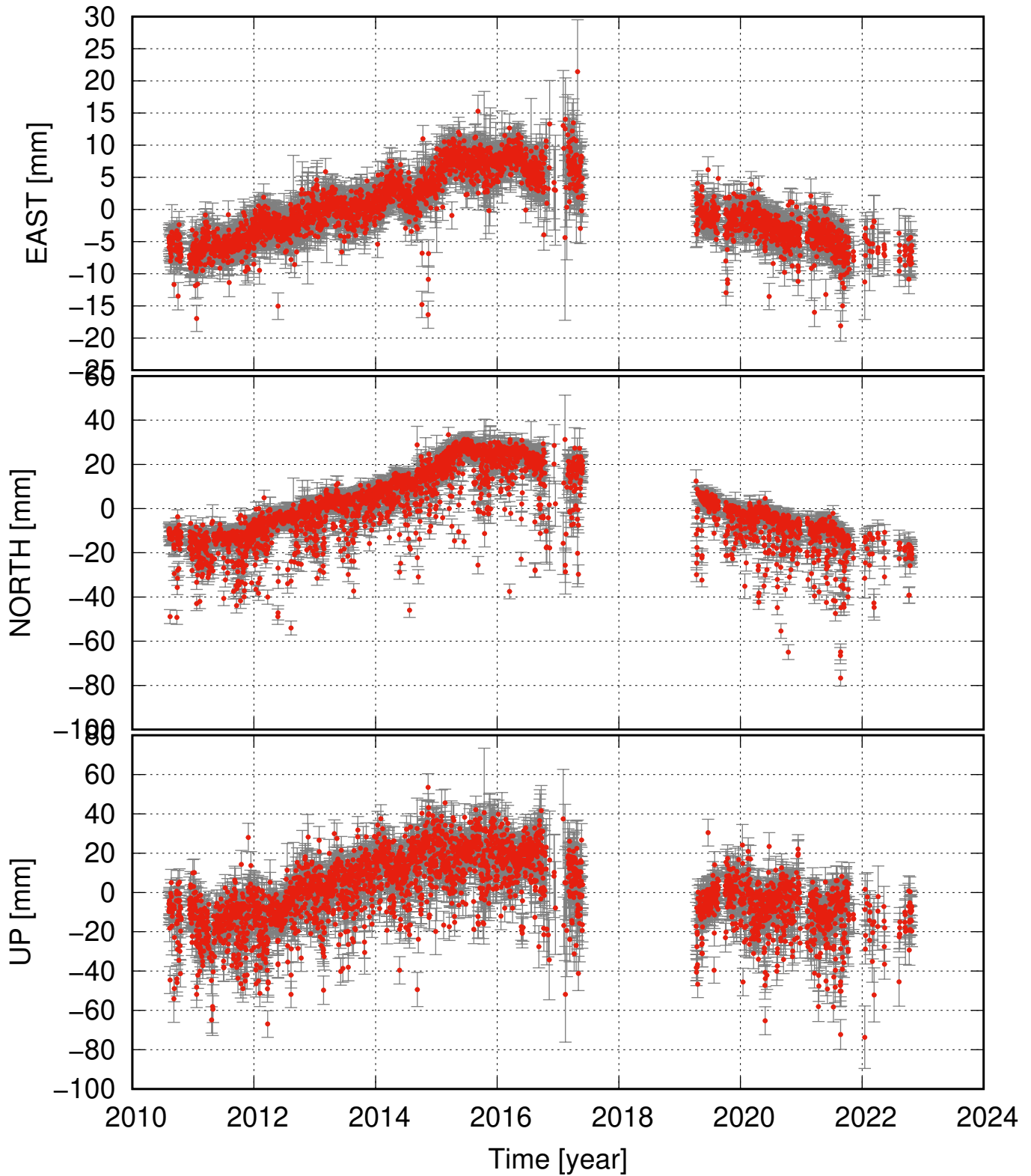
STE2 residual time series (some major events removed as well)
