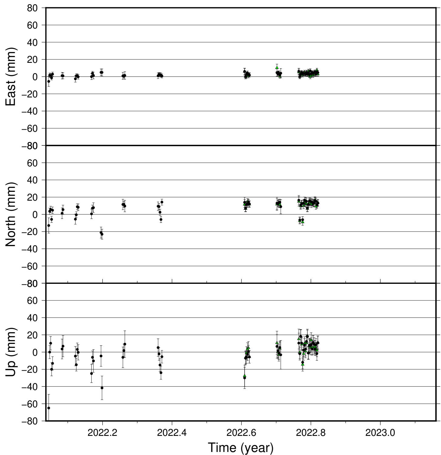
STE2 time series (IGS 2014), last 400 days
