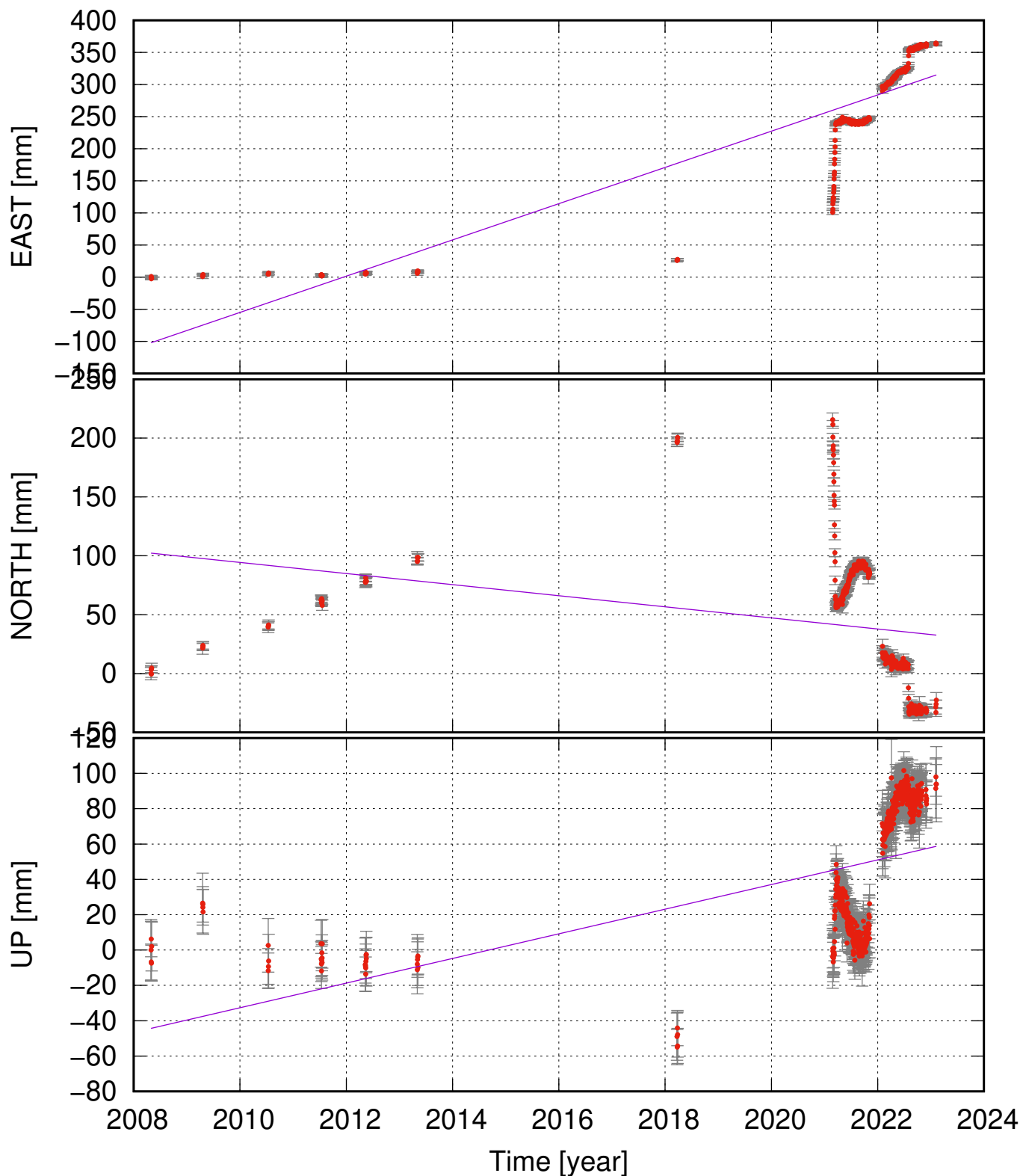
STAN (63.85, -22.23) time series (ITRF 2014) ve = 28.23 ± 2.90; vn = -4.70 ± 3.46; vu = 6.98 ± 2.25 mm/yr
