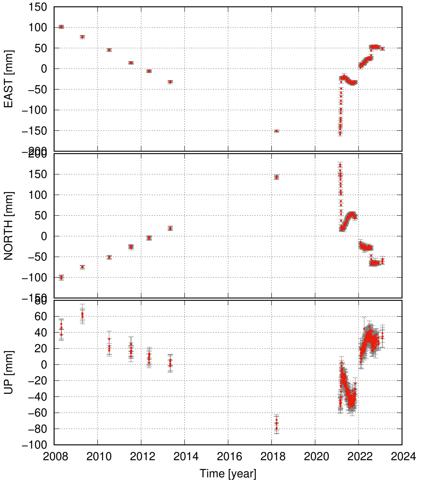
STAN residual time series (some major events removed as well)
