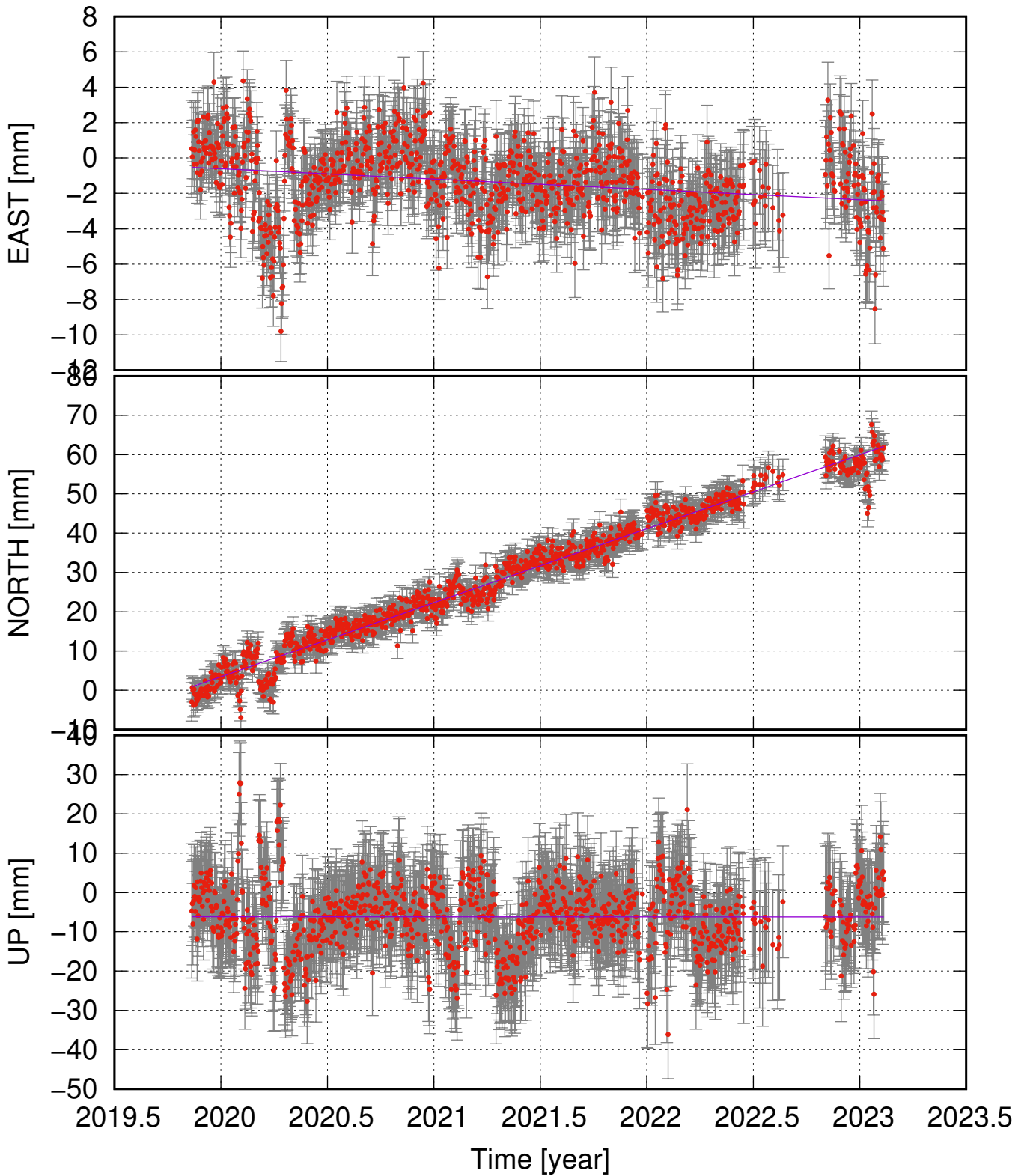
SPBC (65.72, -16.75) time series (ITRF 2014) v_e = -0.58 \pm 0.61 ; v_n = 18.83 \pm 0.86 ; v_u = -0.02 \pm 2.57 mm/yr
