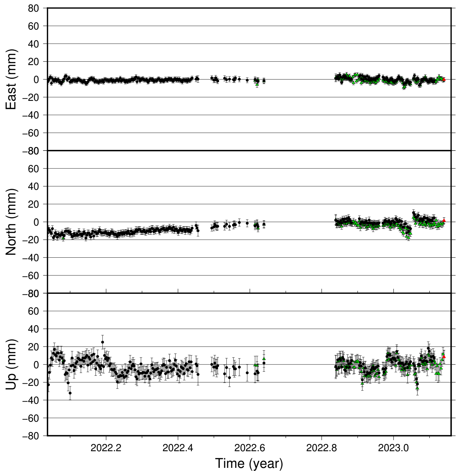
SPBC time series (IGS 2014), last 400 days
